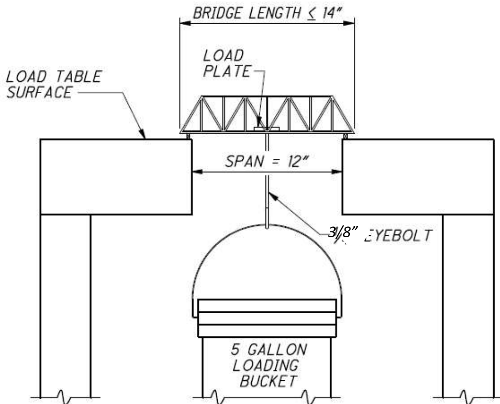
LOADING TABLE SETUP
