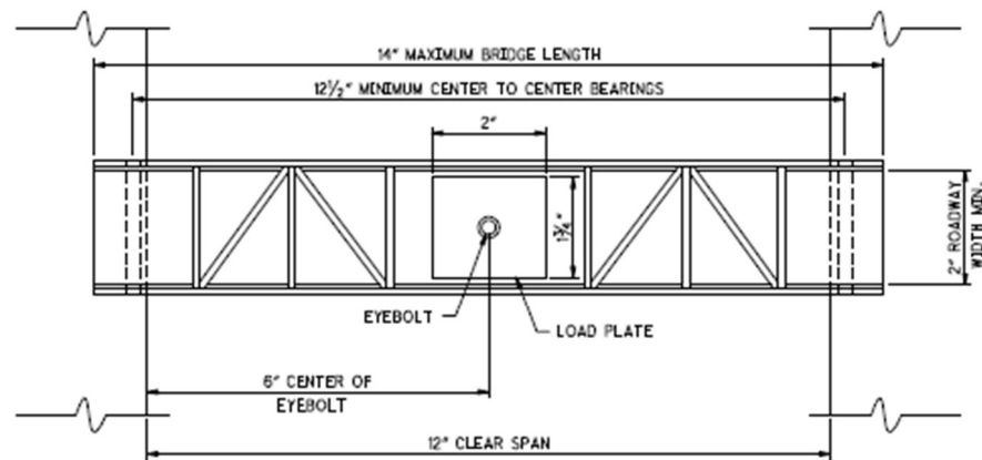
STRUCTURE PLAN
