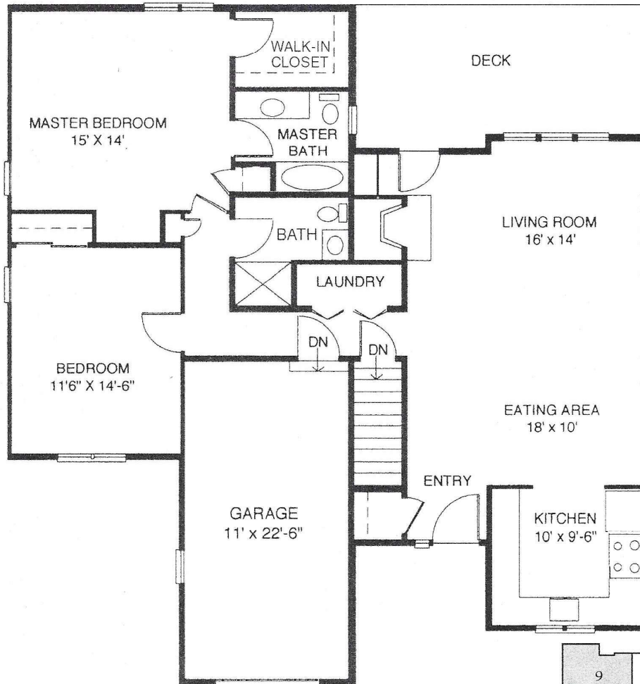
TWO-UNIT BUILDING 9 and 8 are Provincetown Models
