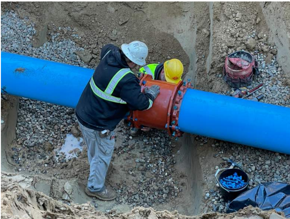
Photo #7: Tying in the force main pipe with a sleeve, near stationing 154+23 alongside Aztec Road - Feb 21, 2024, 10:04 AM
