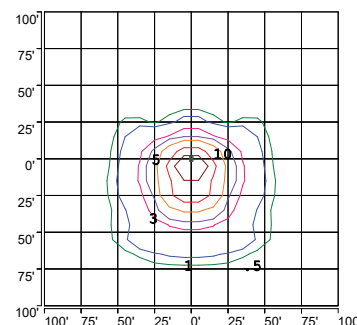
ISOFOOTCANDLE PLOT: DCLB3GP1 1000W MH CENTER COURT SERIES 23' AFG - 0 DEGREE TILT
