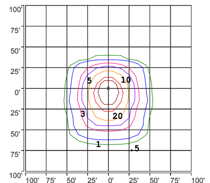
ISOFOOTCANDLE PLOT: AURORA 1000W MH CENTER COURT SERIES 23' AFG - 0 DEGREE TILT
