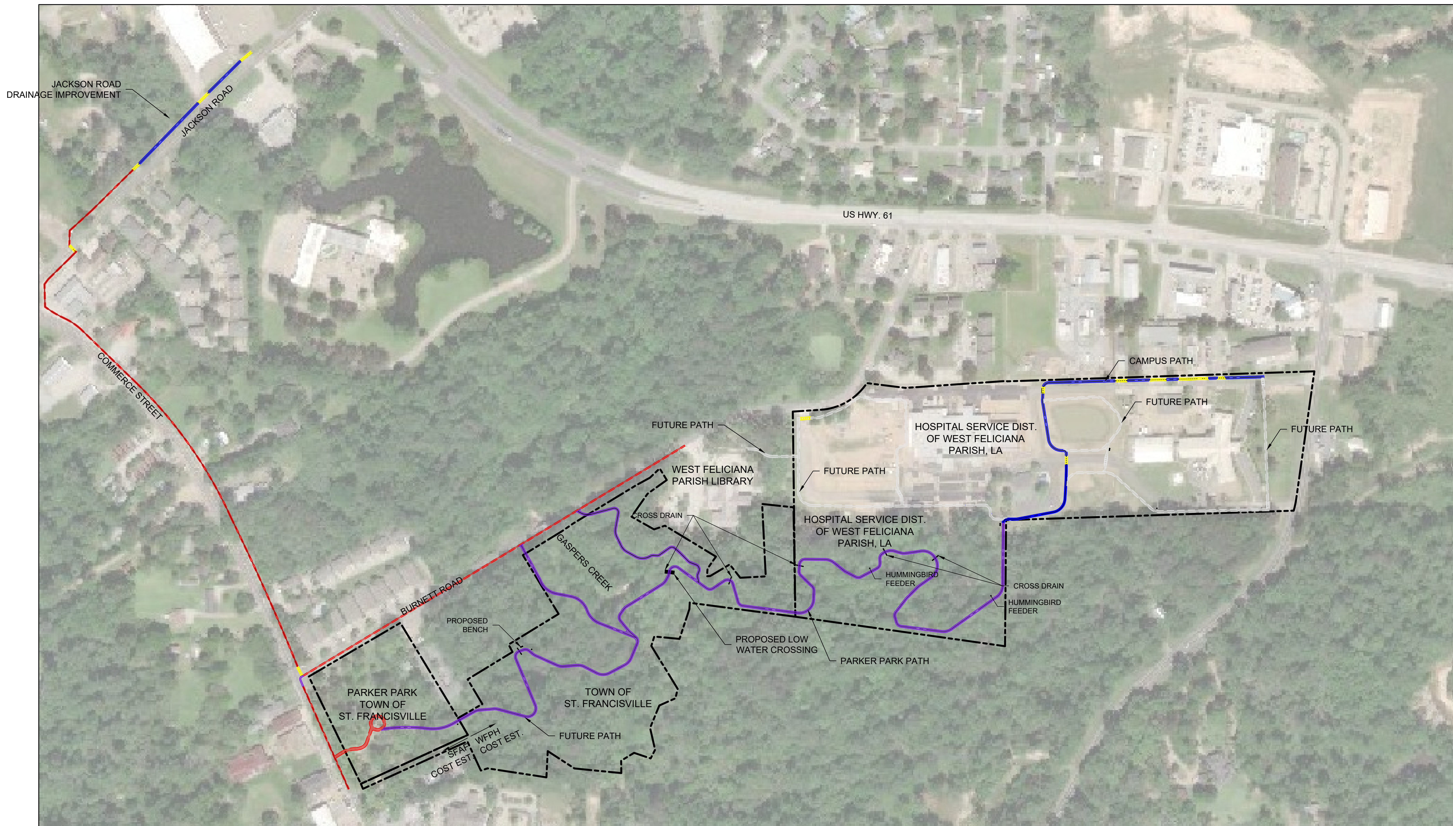
1 PRELIMINARY LAYOUT - SIDEWALK WALKING PATH 1" = 200'
