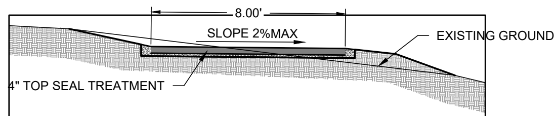
3 PARKER PARK PATH 1" = 5'
