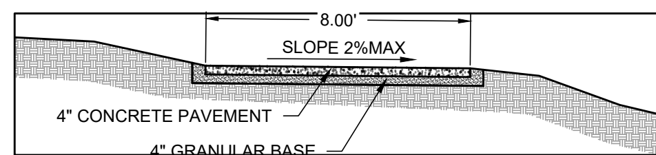
2 CAMPUS PATH CONCRETE PATH 1" = 5'
