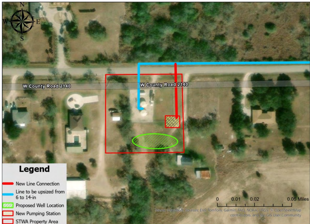
Figure 5B.9.1. STWA Ground Water Well Project Proposed Layout
