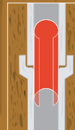
Collar repair with short liner
