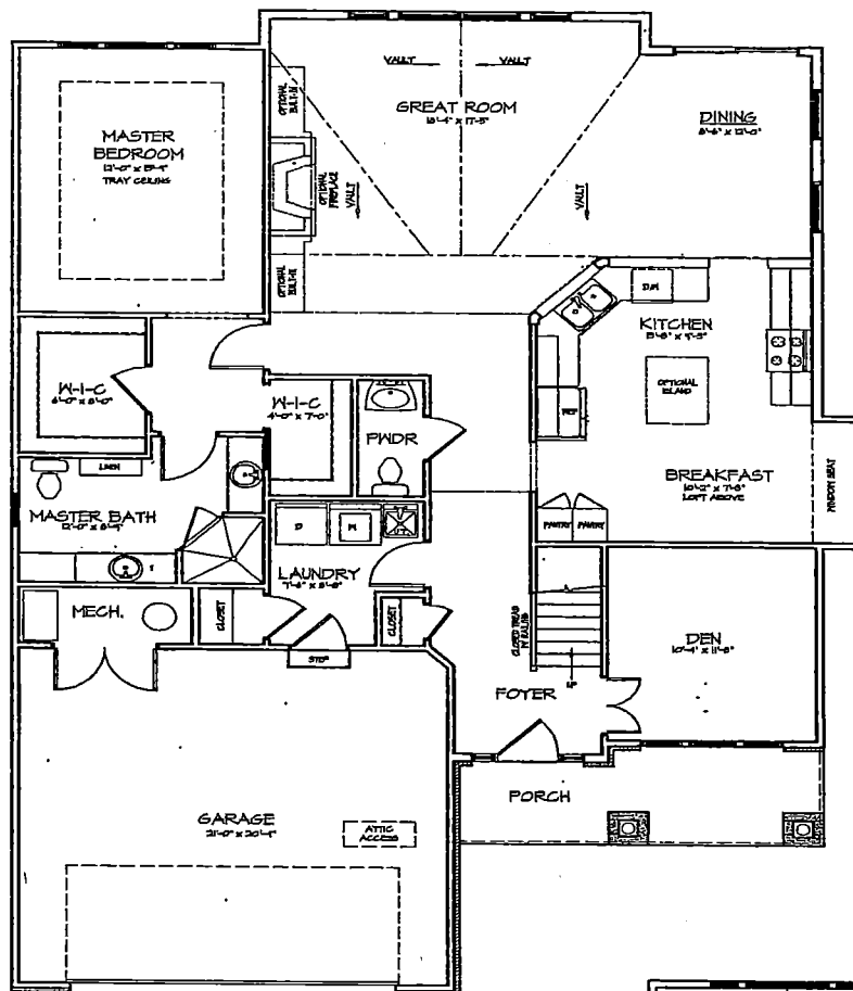
MAIN FLOOR
