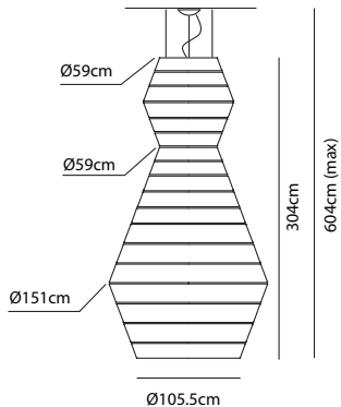
LAYERS B
