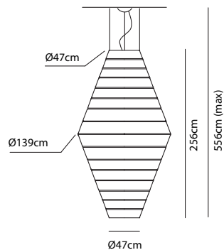
LAYERS C
