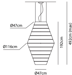
LAYERS D
