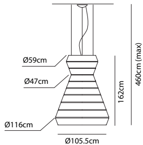
LAYERS A
