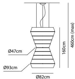
LAYERS F
