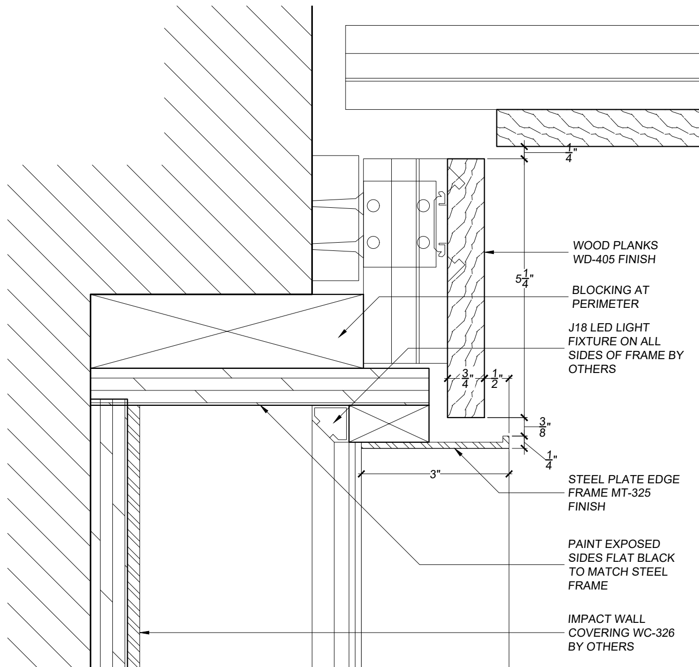
01 2D DETAIL SCALE: 6" - 1'-0" REF.: 7/A802
