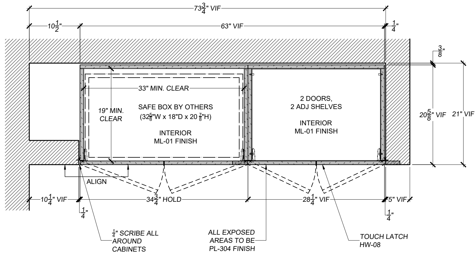
01 3B PLAN SECTION SCALE: 1" = 1'-0" REF.: 1/A802
