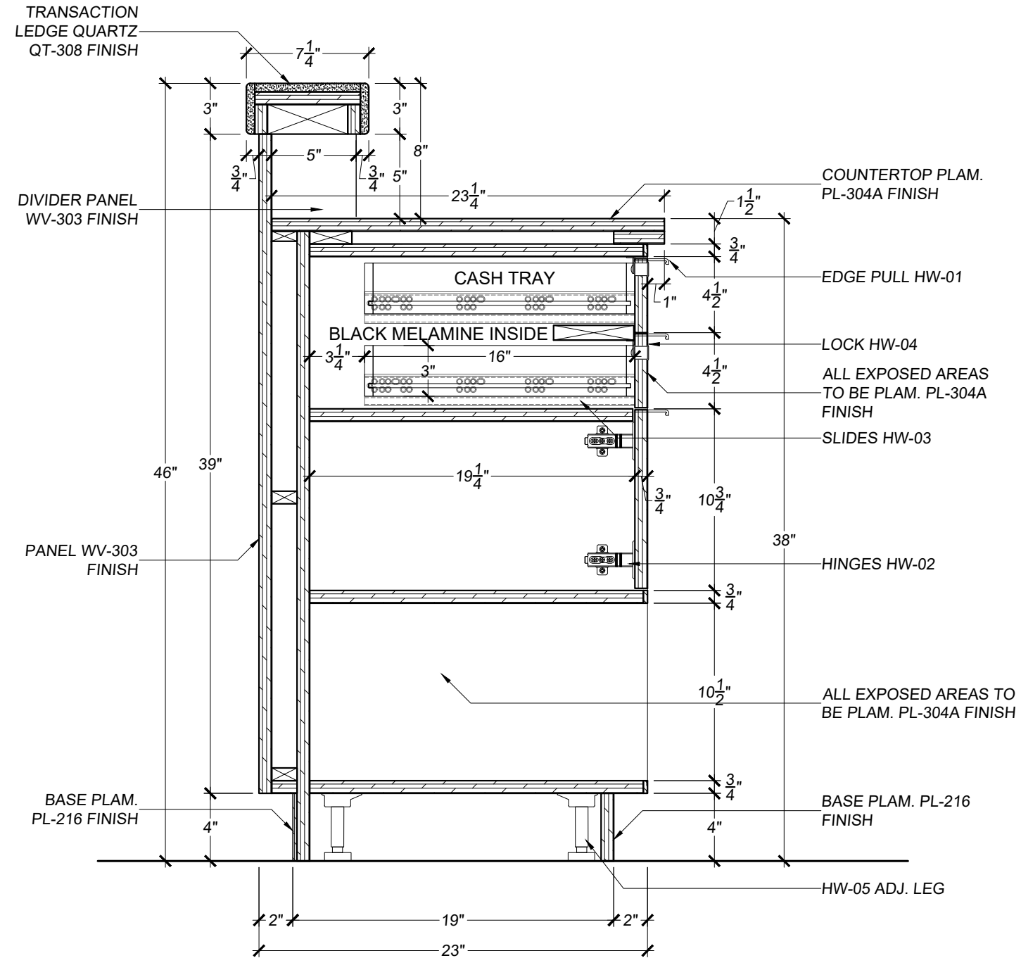
01 SECTION @ CPU CABINET 1G SCALE: 1 1/2" - 1'-0" REF.: 2/A801
