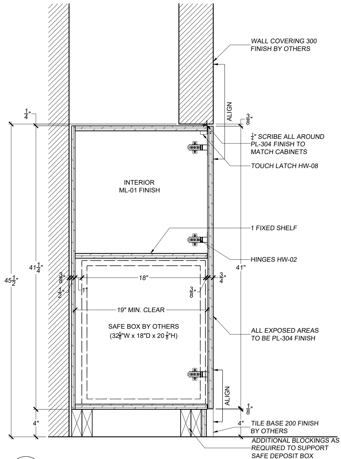
01 VERTICAL SECTION 3C SCALE: 1 1/2" - 1'-0" REF.: N/A
