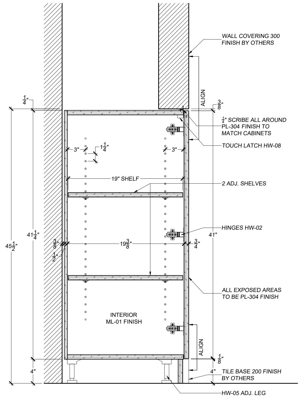
02 VERTICAL SECTION 3C SCALE: 1 1/2" - 1'-0" REF.: N/A
