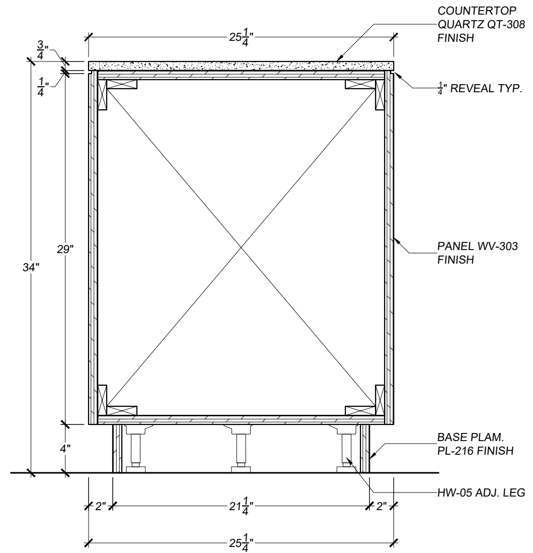
02 SECTION @ ADA TRANSACTION TOP 1H SCALE: 1 1/2" - 1'-0" REF.: 1/A801
