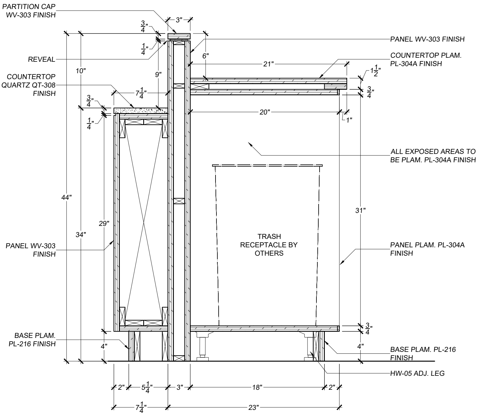
01 SECTION @ TRASH CABINET 1H SCALE: 1 1/2" - 1'-0" REF.: 4/A801
