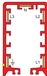
standard 5-pole
