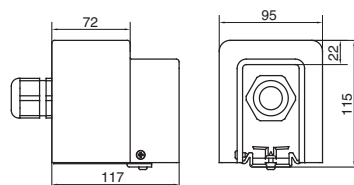
EB40 (opened)
