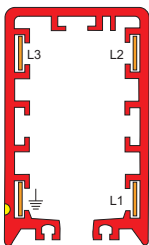
standard 4-pole
