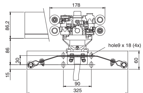
CL7-7-35 + MVSP
