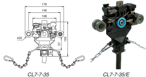
CL7-7-35
