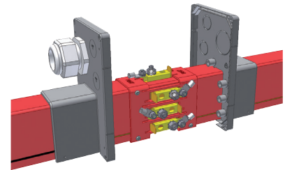
LCH + LC80
