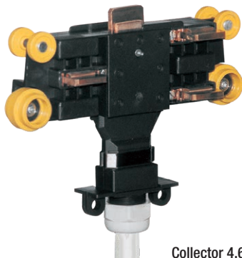
Collector 4,6 and 7 poles
