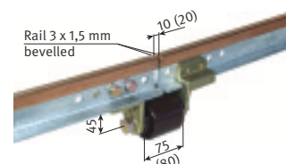
Value in brackets for 20 mm air gap
