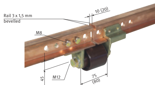
Measures in brackets for 20 mm air gap
