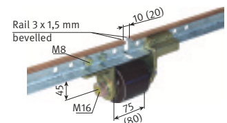
Measures in brackets for 20 mm air gap
