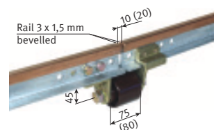
Value in brackets for 20 mm air gap
