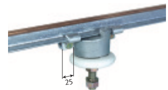
Illustration shows an insulator with 2 locating clamps (fix point)
