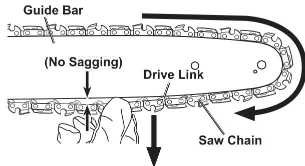
Figure I: Checking Saw Chain Tension
