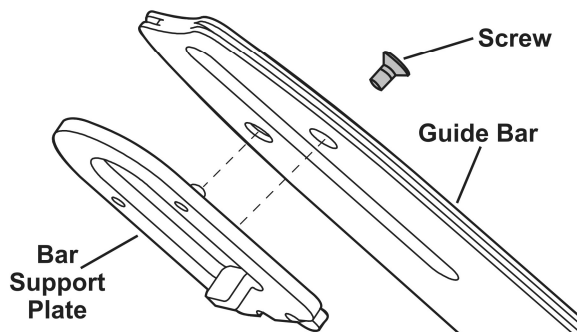
Figure C: Attach Bar Support Plate
