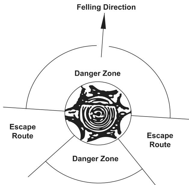
Figure J: Escape Routes
