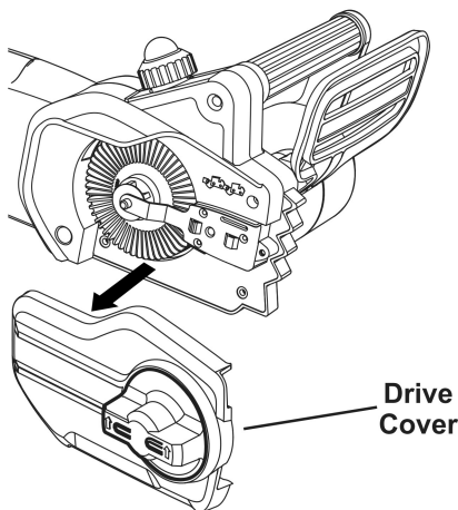
Figure B: Drive Cover Removed
