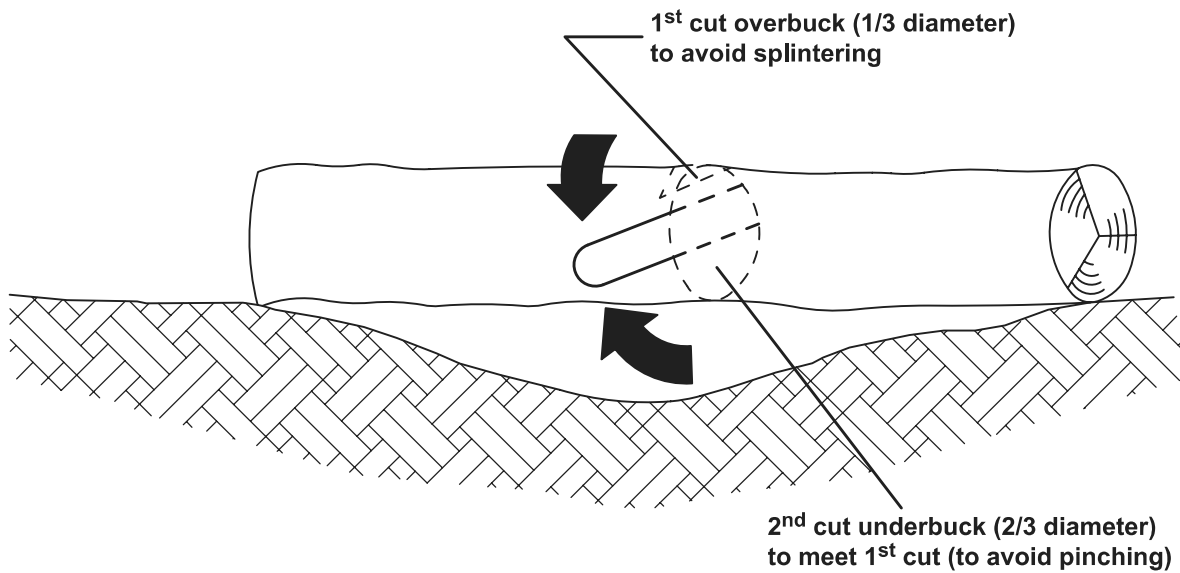
Figure O: Log Supported Both Ends
