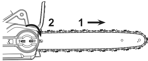
Figure G: Pull Guide Bar Forward
