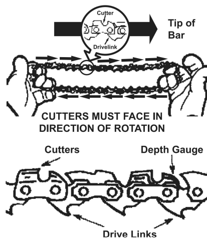
Figure D: Place Saw Chain
