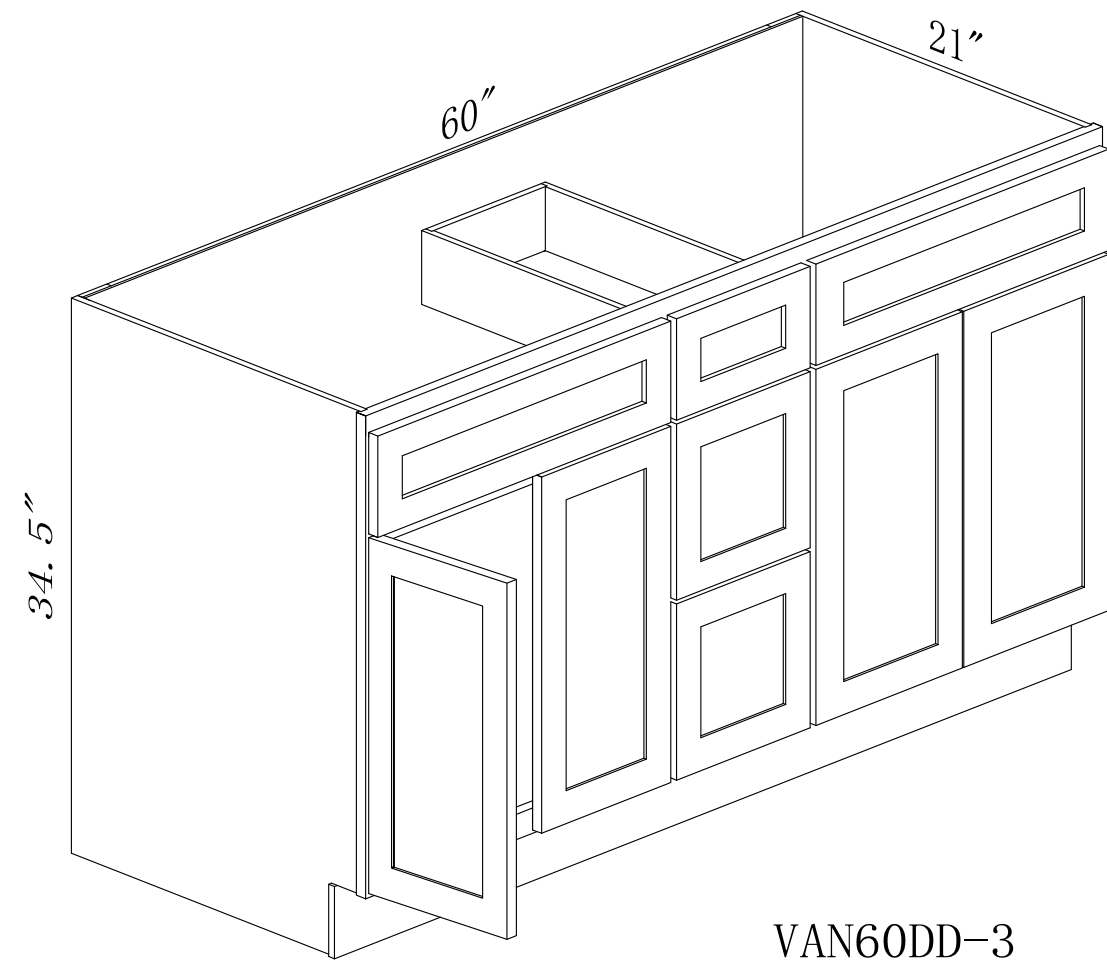
VAN60DD-3 VAN60D-3 (2 sink)
