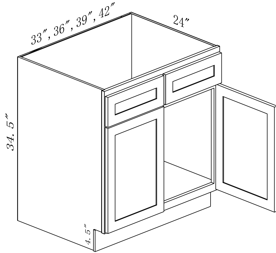
SB33, SB36, SB39, SB42
