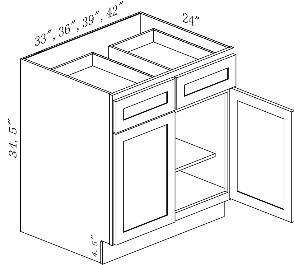
B33, B36, B39, B42
