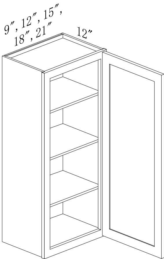
W0942, W1242, W1542 W1842, W2142
