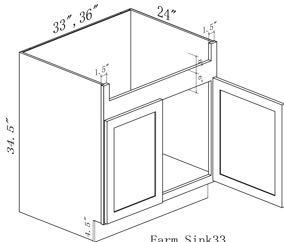
Farm Sink33 Farm Sink36
