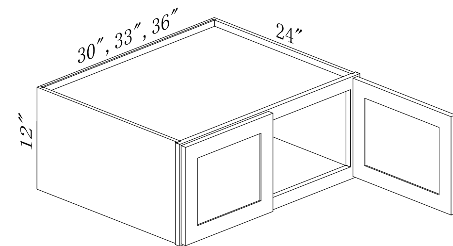
W301224, W331224, W361224
