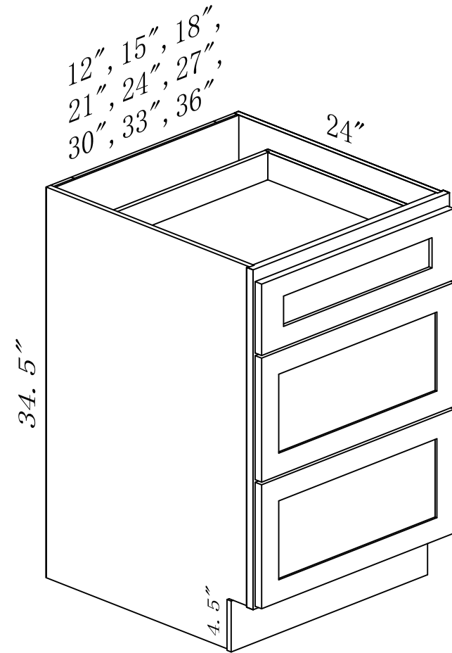
DB12, DB15, DB18, DB21 DB24, DB27, DB30, DB33 DB36
