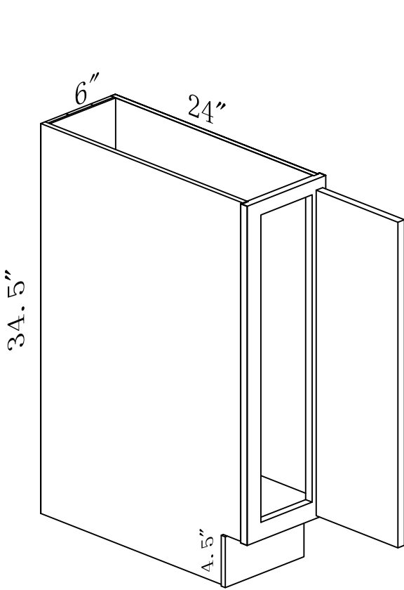
B06 full door
