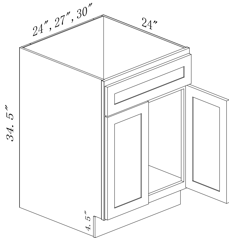
SB24, SB27, SB30
