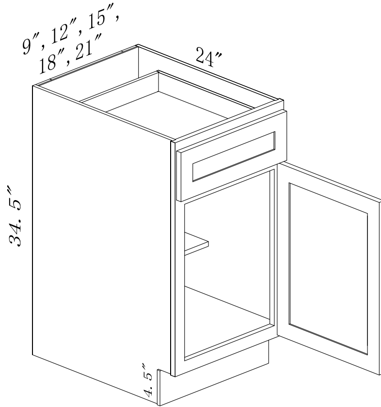
B09, B12, B15 B18, B21
