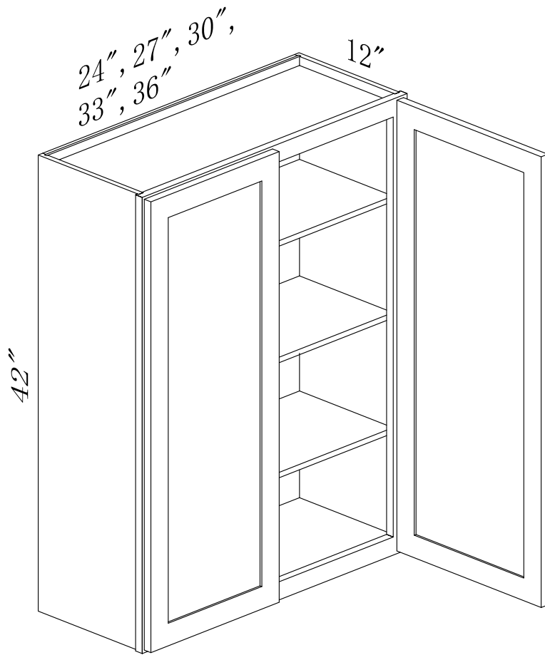
W2442, W2742, W3042 W3342, W3642
