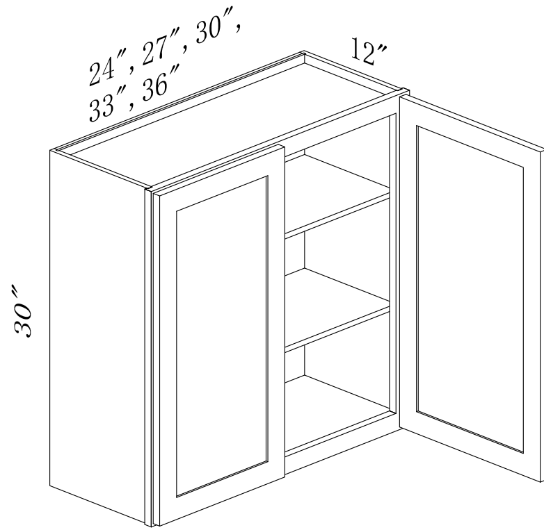
W2430, W2730, W3030 W3330, W3630
