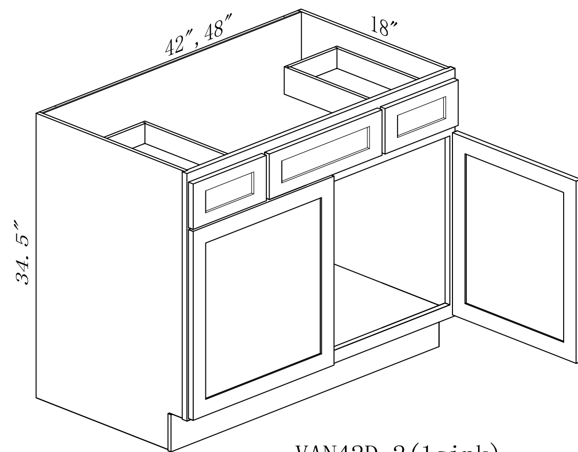
VAN42D-2 (1sink) VAN48D-2 (1sink)
