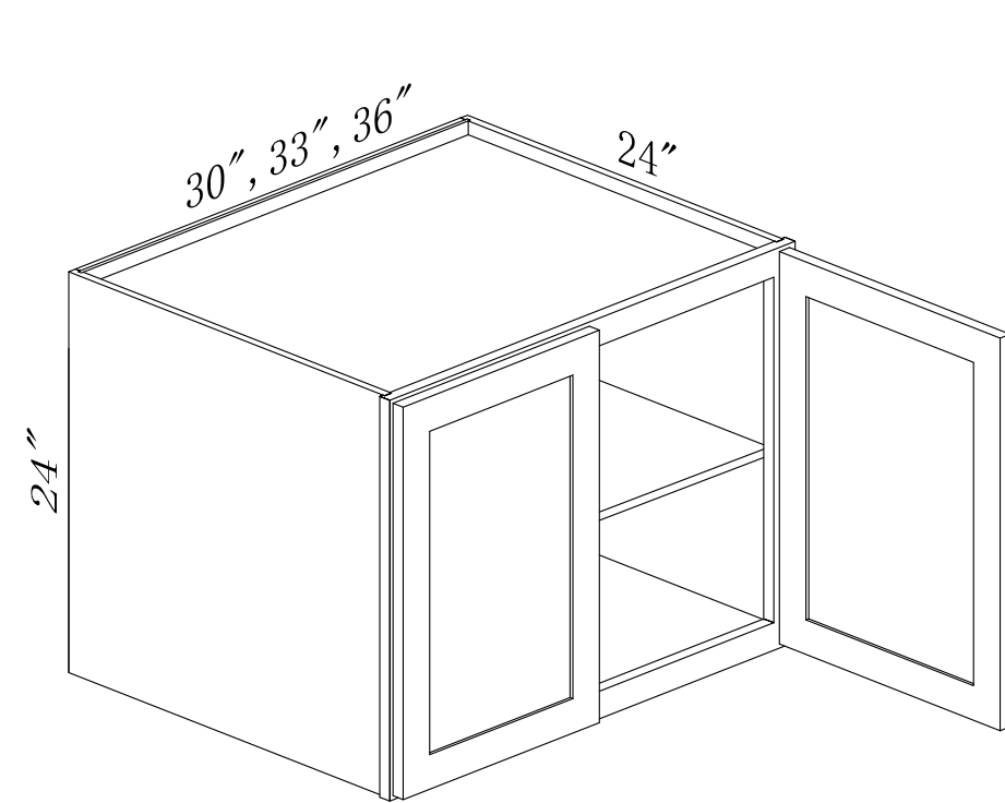
W302424, W332424, W362424
