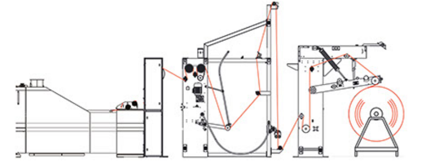
Non Stop J-Box + Dok Sarıcı / Non Stop J-Box + Big Batch
