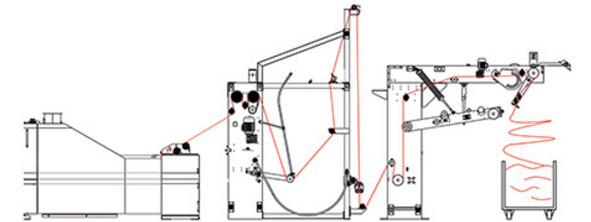
Non Stop J-Box + Pastal Serme + Dok Sarıcı / Non Stop J-Box + Plater + Big Batch
