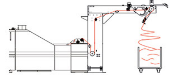
Pastal Serme / Plater
