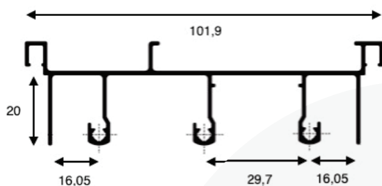
EXM-37 - 1,056 kg/m
