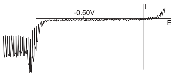
F4. DC polarogram of 2 mM NADP + and 2 mM NADPH in EBS. E_i = 0.260\text{V} , E_f = -1.24\text{V} , scan rate = 5 mV/s, t = 1\text{ s} .
