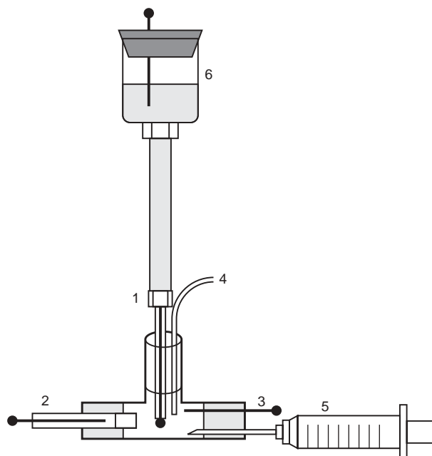
F2. Micropolarographic cell, V=500 \mu\text{L} . 1) DME; 2) Reference electrode; 3) \text{C}^\circ auxiliary electrode; 4) nitrogen inlet; 5) \text{Hg}^\circ purge; 6) \text{Hg}^\circ pool.
