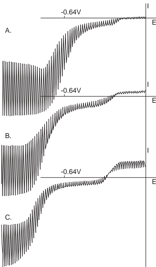
F5. Evolution of DC polarograms of 2 mM GSSG, 20 mM NADPH in EBS and 1 mM EDTA with 5 \mu\text{L} of GR stock solution. a) 0 min; b) 26 min; and c) 30 min. of enzymatic action.
