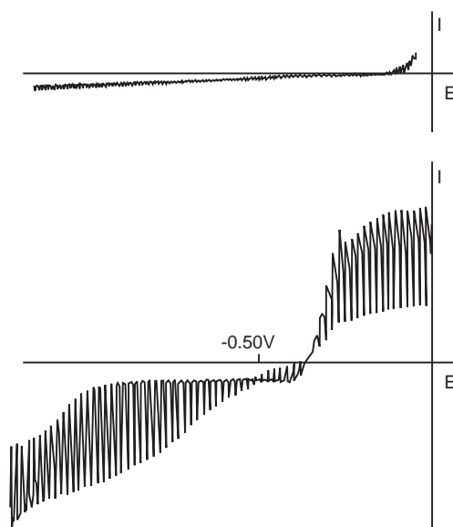
F3. DC polarograms of a) Buffer Electrolyte Solution, BSE: 10 mM Tris \text{pH} = 8.0 , \text{KNO}_3 100 mM; b) 1.45 mM GSSG and 2 mM GSH in EBS. E_i = 0.260\text{V} , E_f = -1.24\text{V} , scan rate = 5 mV/s, t = 1 s.
