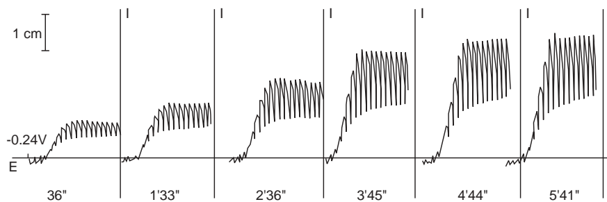
F6. GSH production due to enzymatic activity, EA. Sampling time is indicated below polarograms.
