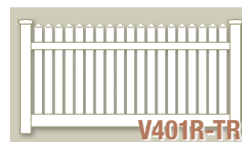
7/8" X 3" PICKETS WITH POINTED PICKET CAPS (REDUCED SPACING)
