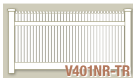
7/8" X 1-1/2" PICKETS W/ POINTED PICKET CAPS (REDUCED SPACING)
