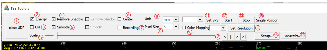
FIG 2.2 Main User Controls Area
