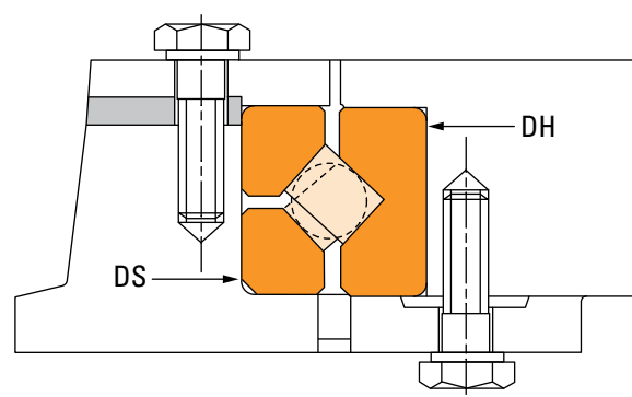
Fig. 82. Fitting and setting of TXR bearings.
