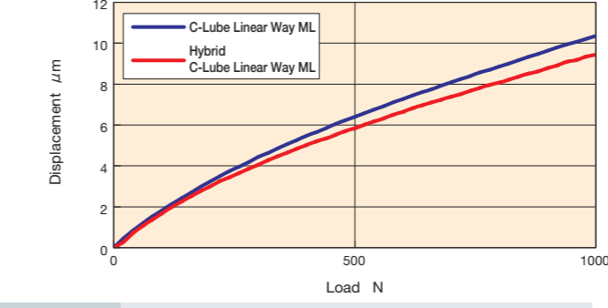
Test conditions Model : ML12 Preload: Standard Preload Load direction: Downward
