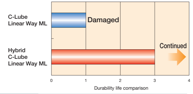
Test conditions Model : ML12 Velocity: 300 m/min Acceleration: 40 G
