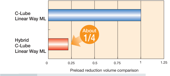
Test conditions Model : ML12 Velocity: 300 m/min Acceleration: 40 G Traveling distance: 13,000 km
