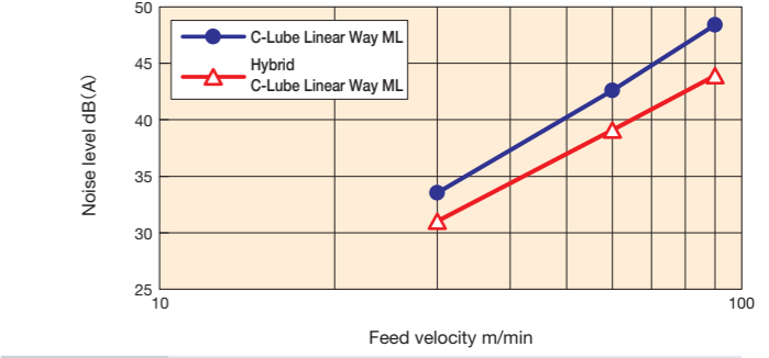
Test conditions Model : ML12 Measurement velocity: 30, 60, 90 m/min
