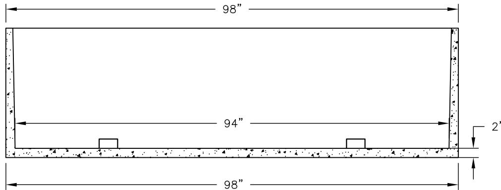
SECTION "B" CONCRETE GRAVE LID
