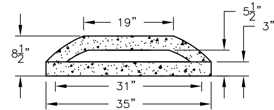
SECTION "B" EPOXY LINED LID
