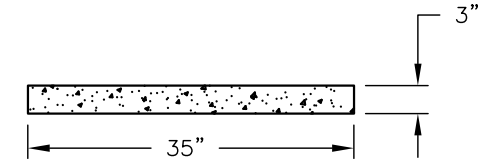
SECTION "B" ETHNIC BURIAL LID
