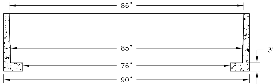
FRONT VIEW SECTION "A"
