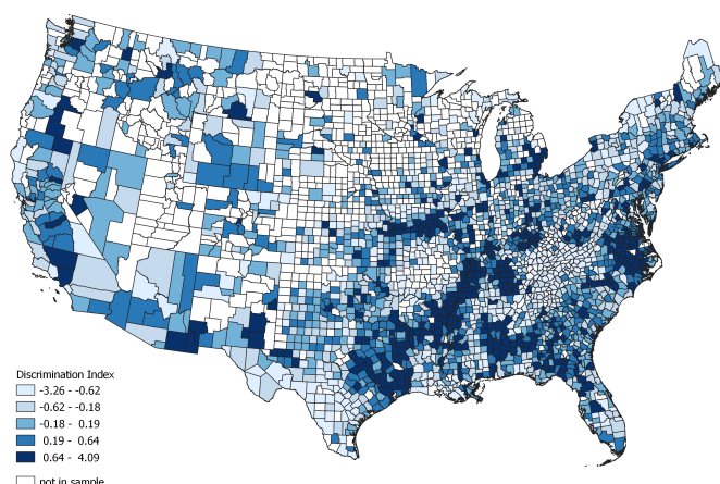
Figure A.1: Discrimination (within State Variation)
