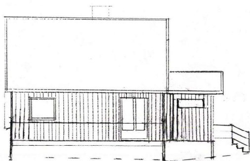
FASADE VEST.
