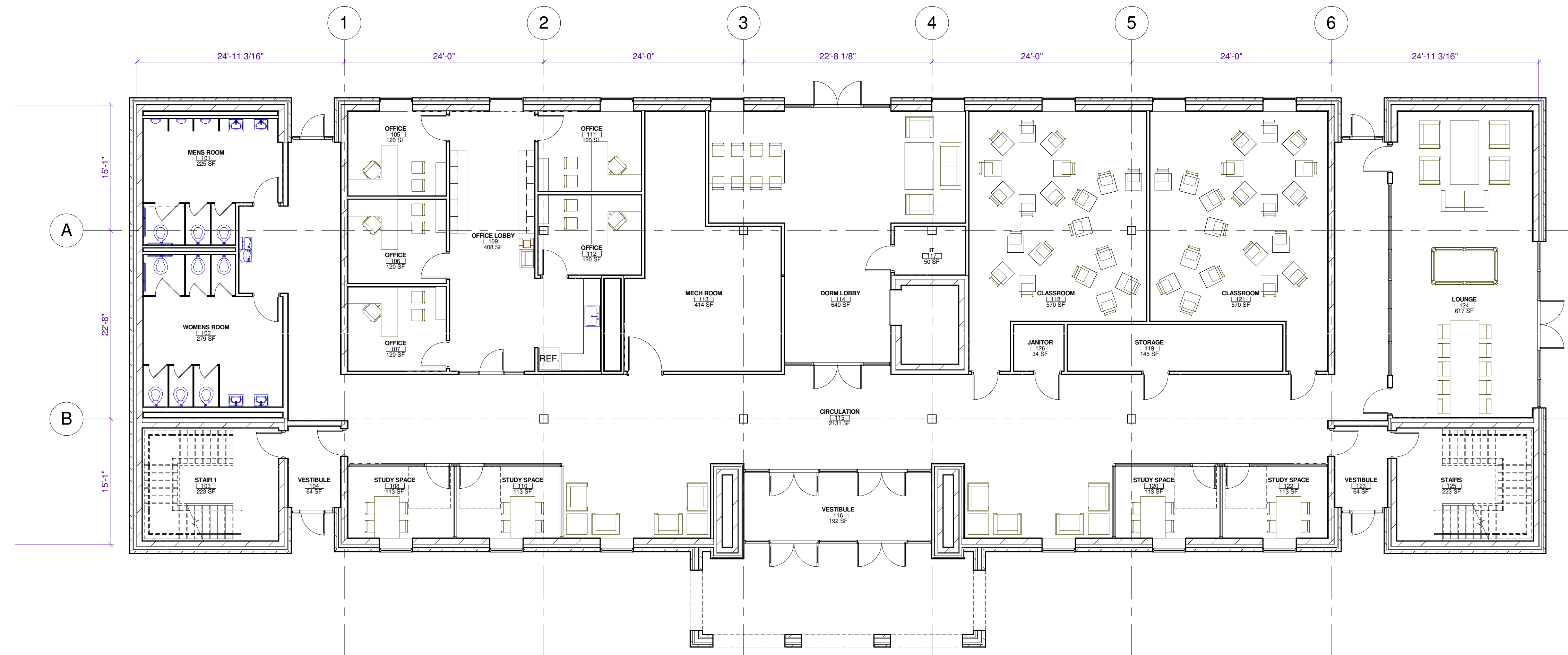
FIRST FLOOR ARCHITECTURAL PLAN 1/8" = 1'-0"
