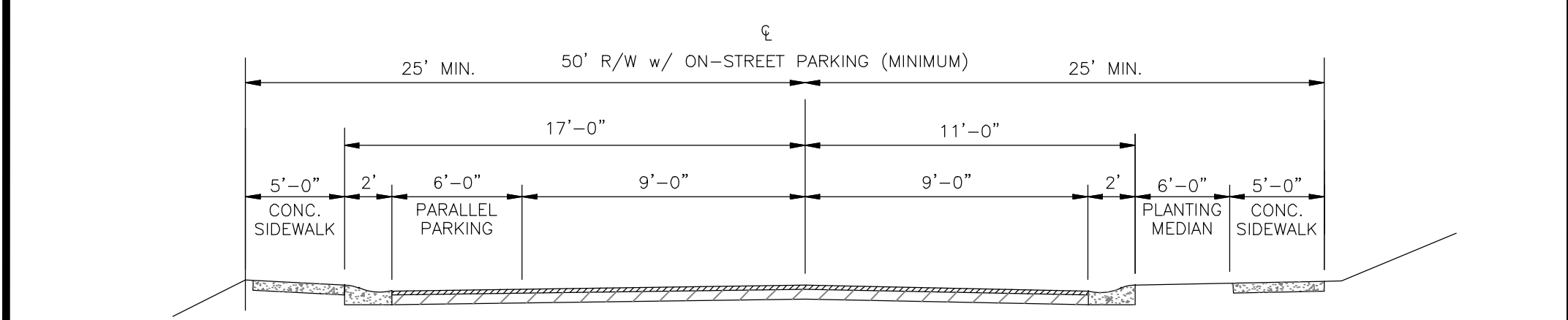
50' Public ROW (with On-Street Parking)
