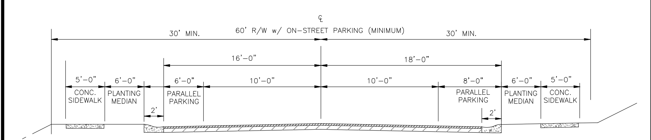
60' Public ROW (with On-Street Parking)
