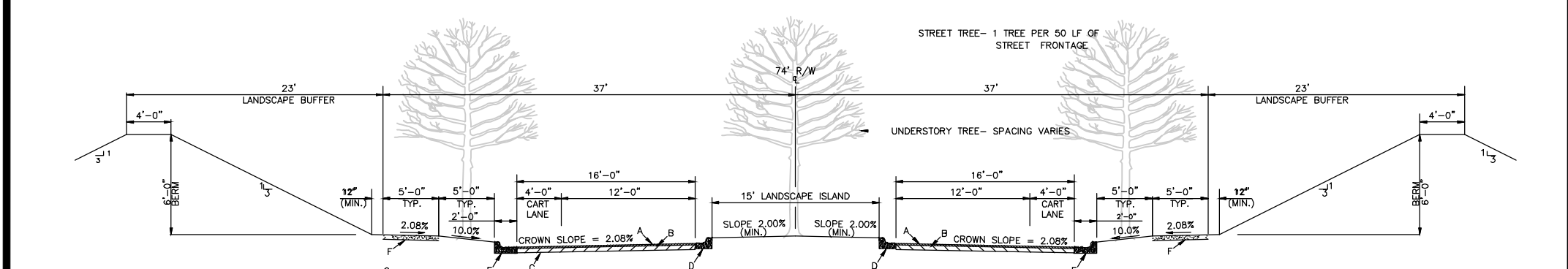
120' Belmont/Mt.Holly Connector ROW
