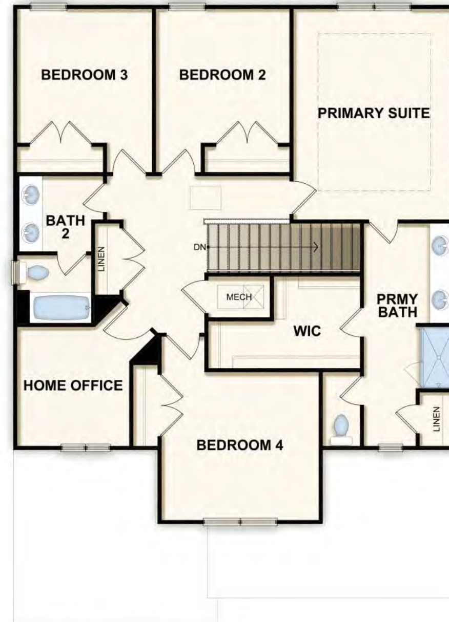
SECOND FLOOR PLAN BASE ELEVATION SHOWN
