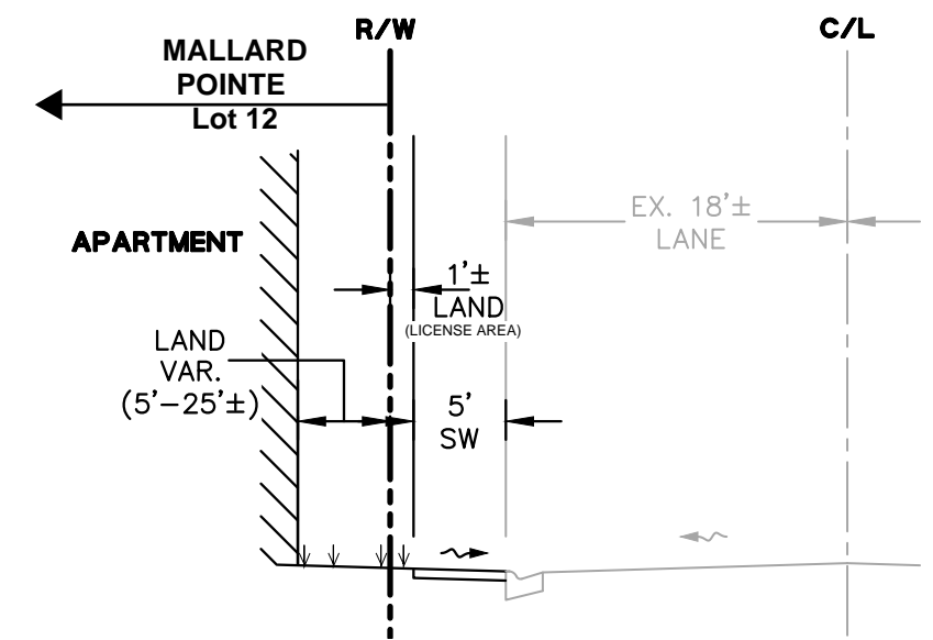
SECTION A NTS
