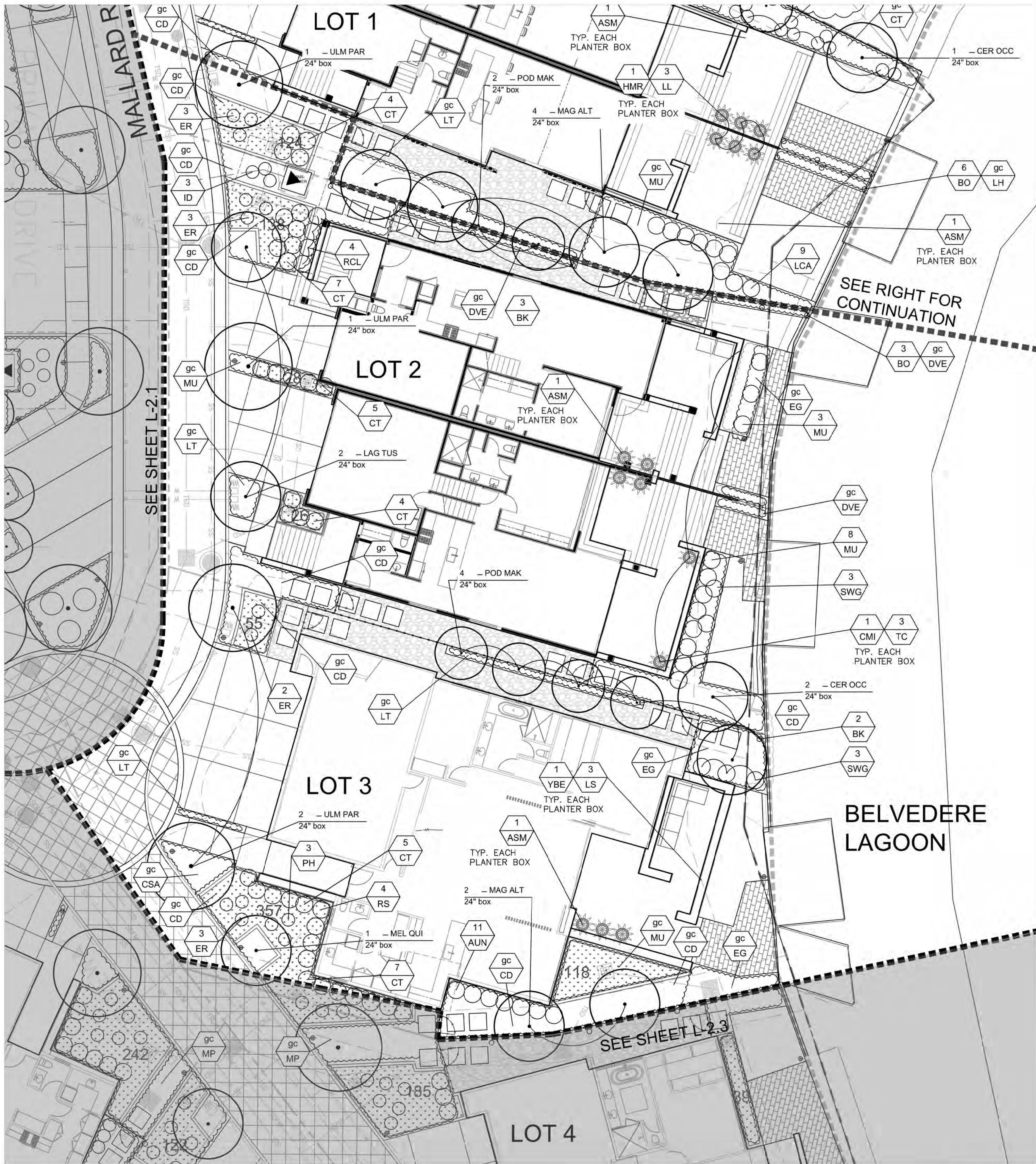
PLANTING PLAN
