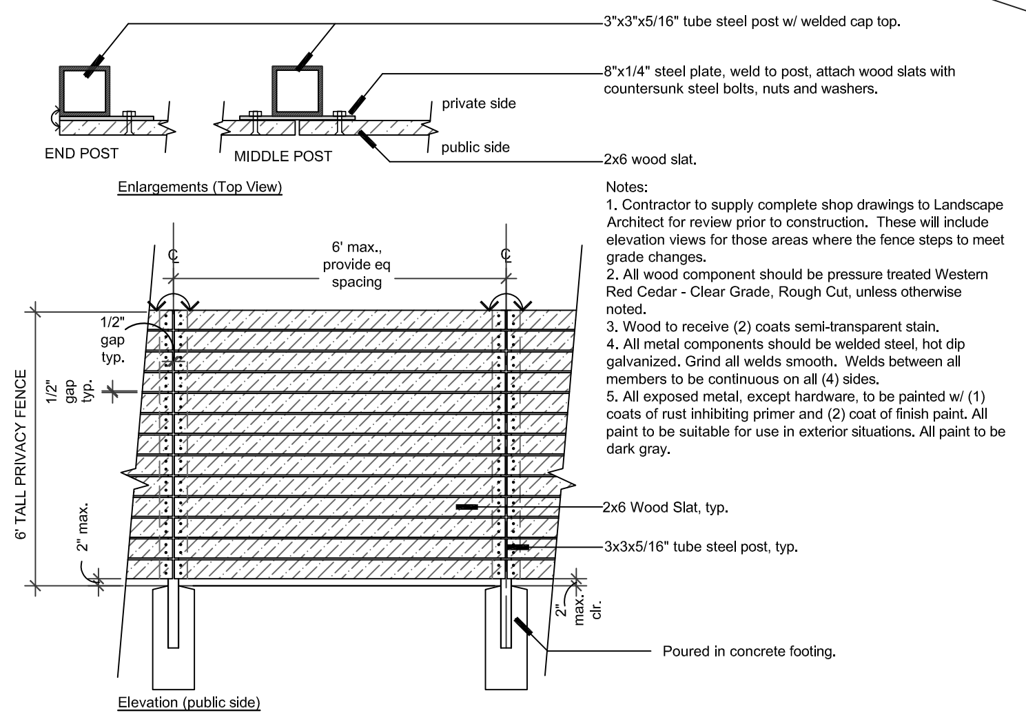
Horizontal Wood Fence scale: 3/8"=1'-0"
