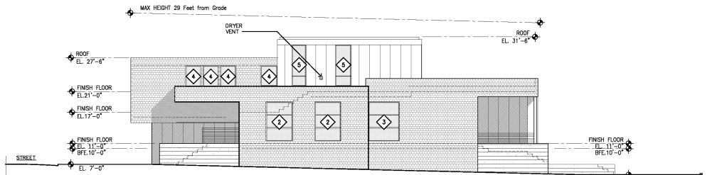
East Elevation Scale 1"=8'-0"
