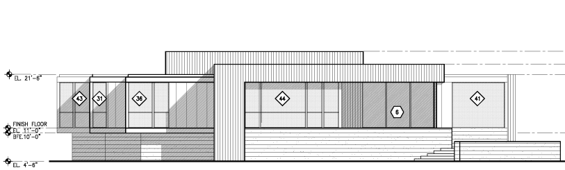
North Elevation Scale 1"=8'-0"
