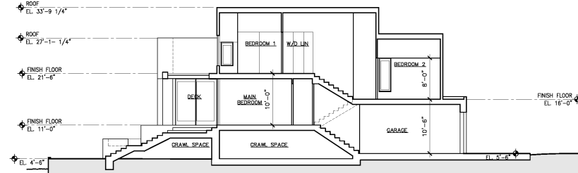
Building Section 2 Scale 1"=8'-0"
