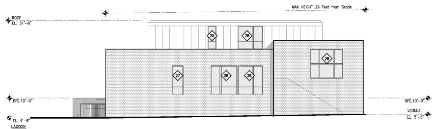
West Elevation Scale 1"=8'-0"
