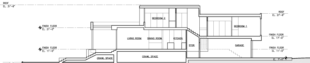
Building Section 1
