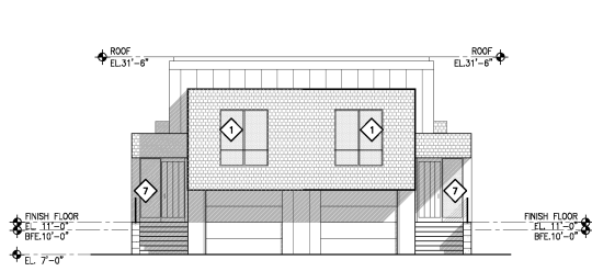
South Elevation Scale 1"=8'-0"
