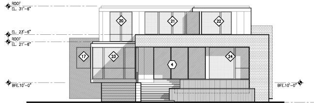
North Elevation Scale 1"=8'-0"
