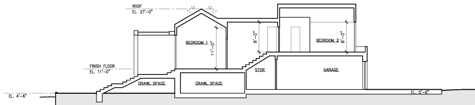
Building Section 1 Scale 1"=8'-0"
