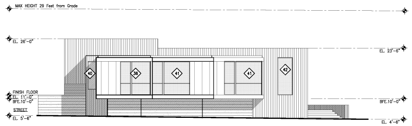
East Elevation Scale 1"=8'-0"
