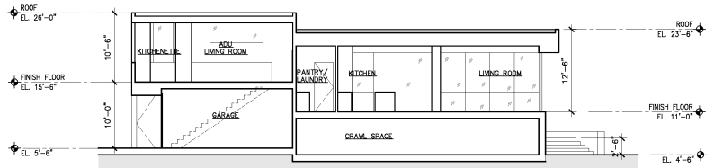
Building Section 1 Scale 1"=8'-0"
