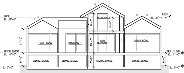
Building Section 4 Scale 1"=8'-0"
