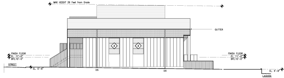
East Elevation Scale 1"=8'-0"
