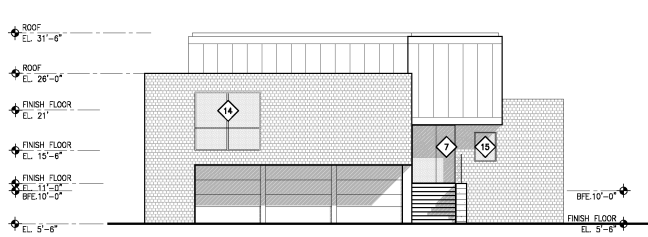
South Elevation Scale 1"=8'-0"
