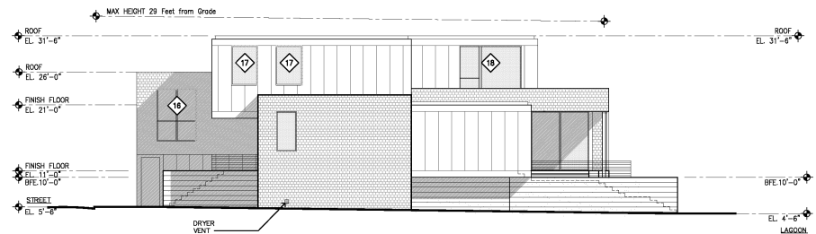
East Elevation Scale 1"=8'-0"
