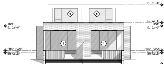
North Elevation
