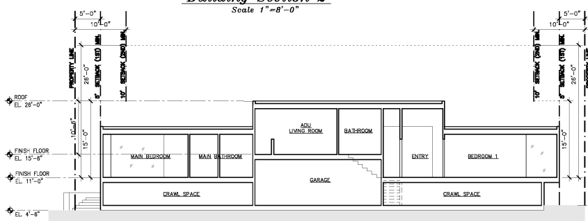
Building Section 3 Scale 1"=8'-0"
