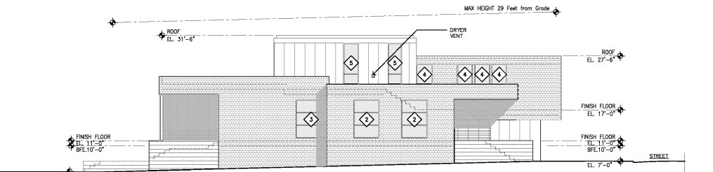
West Elevation Scale 1"=8'-0"
