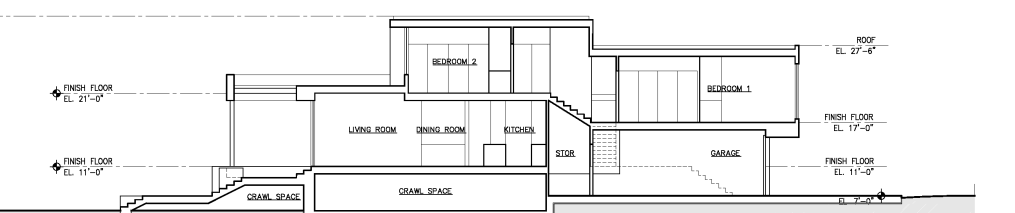
Building Section 1 Scale 1"=8'-0"
