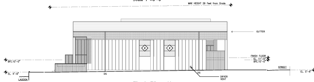
West Elevation Scale 1"=8'-0"
