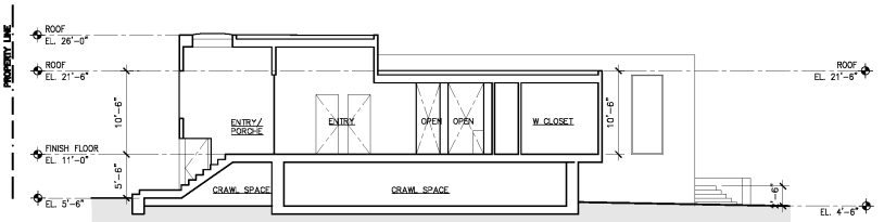
Building Section 2 Scale 1"=8'-0"
