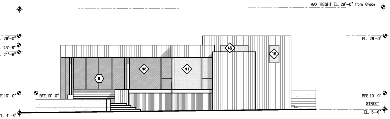
West Elevation Scale 1"=8'-0"
