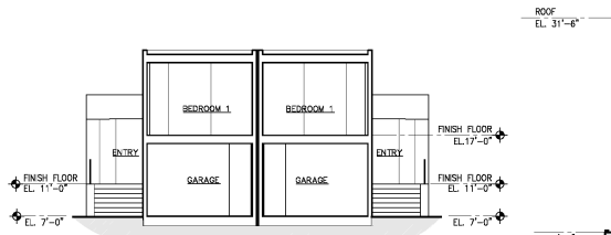
Building Section 2 Scale 1"=8'-0"
