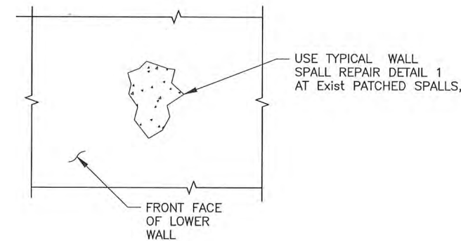
4 CONCRETE PATCH REPAIR No scale
