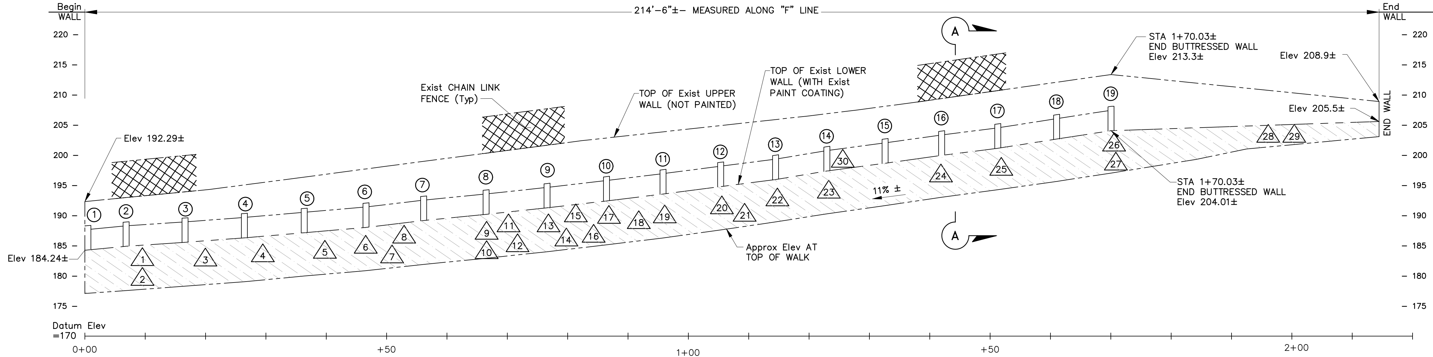
ELEVATION - EXISTING RETAINING WALL SCALE: 1"=10'
