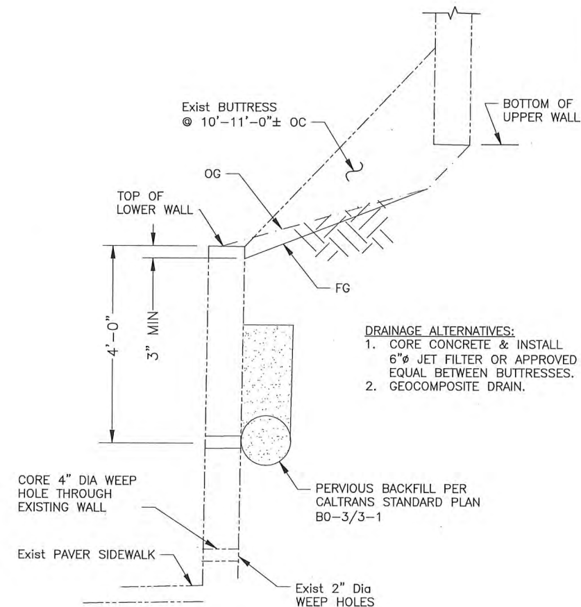
5 DETAIL - WEEP HOLE AND PERVIOUS BACKFILL 3/4"=1'-0"
