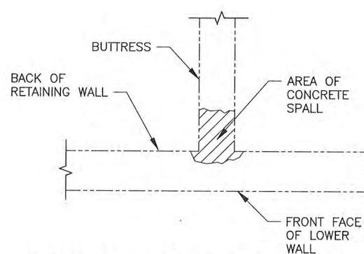
3 PLAN - BUTTRESS/WALL SPALL REPAIR No scale
