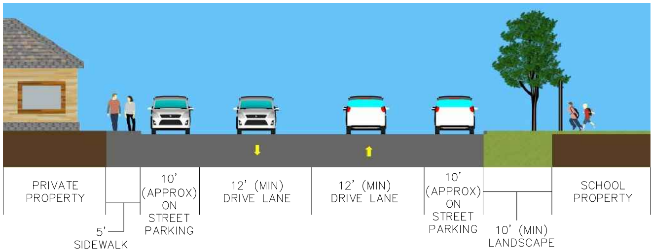
EXISTING CONDITIONS FOR PEAR AND ALMOND STREETS
