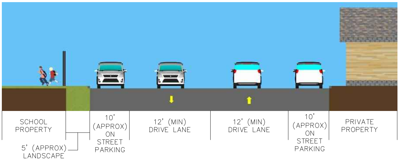
EXISTING CONDITIONS FOR FIG STREET
