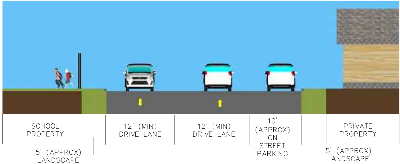
EXISTING CONDITIONS FOR FIG STREET AT ALMOND STREET
