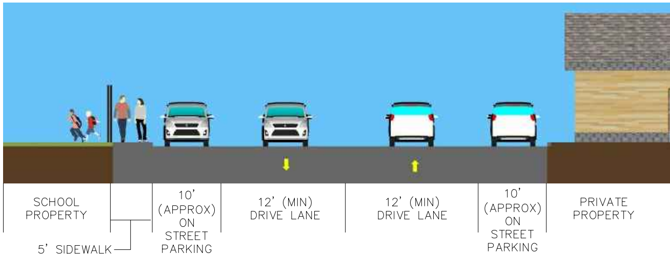
PROPOSED CONDITIONS FOR FIG STREET
