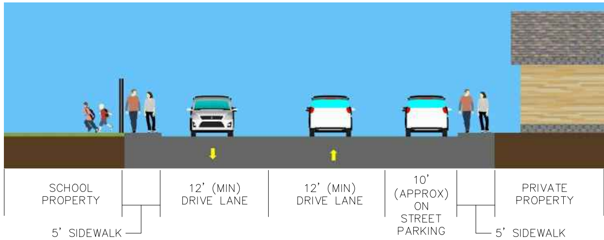
PROPOSED CONDITIONS FOR FIG STREET AT ALMOND STREET
