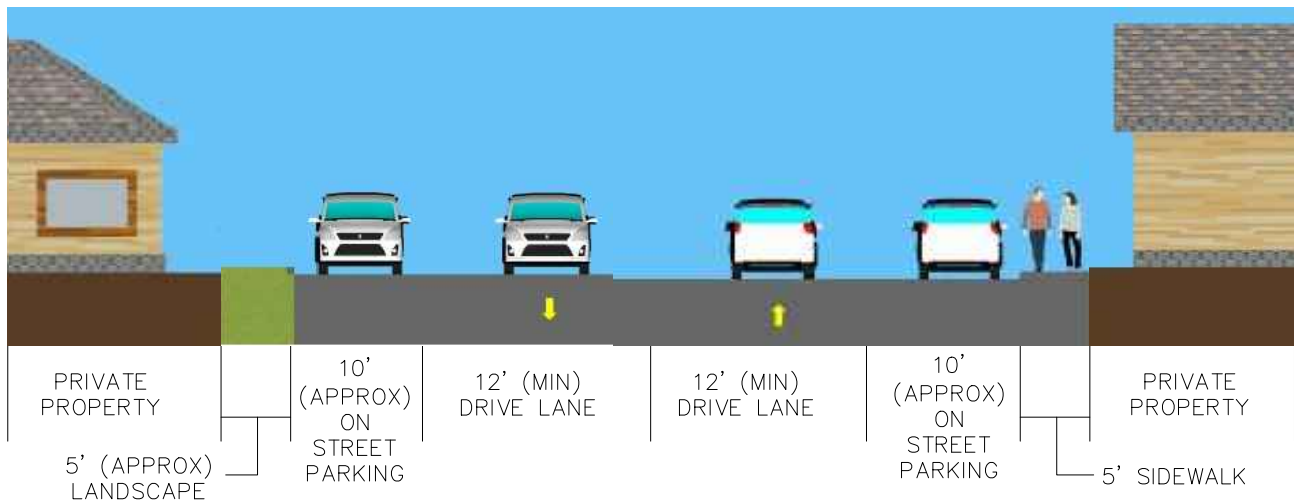
PROPOSED CONDITIONS FOR ALMOND STREET BETWEEN FIG AND MARGUERITE STREETS
