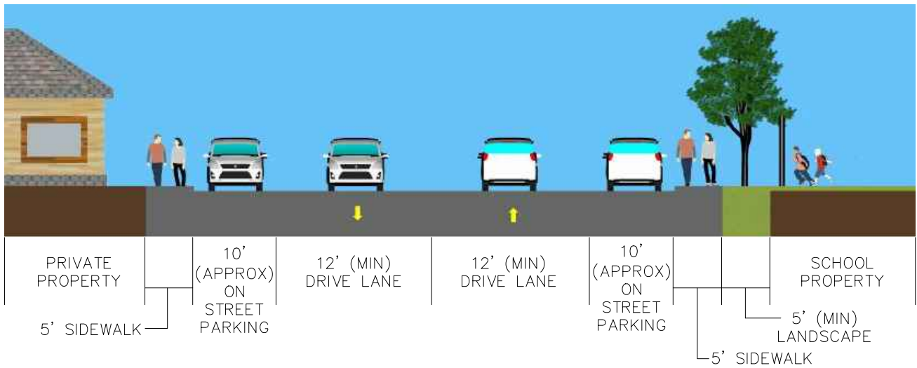
PROPOSED CONDITIONS FOR PEAR AND ALMOND STREETS
