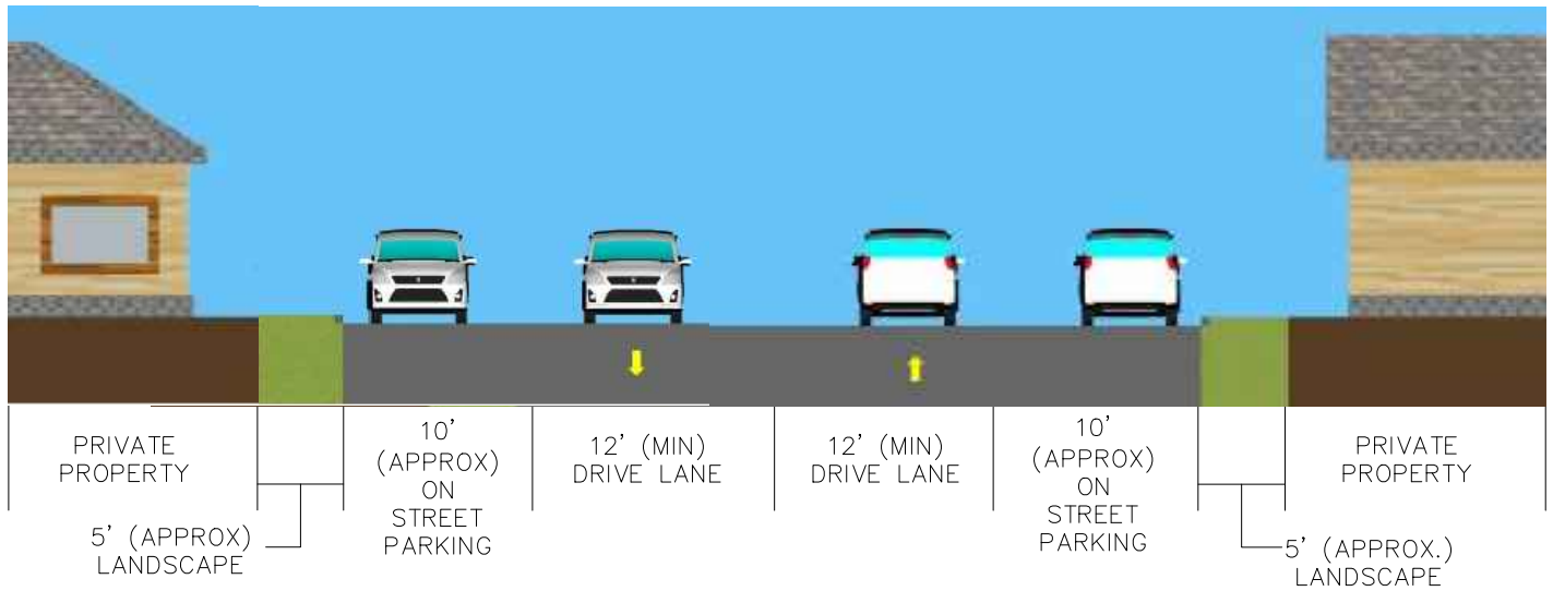
EXISTING CONDITIONS FOR ALMOND STREET BETWEEN FIG AND MARGUERITE STREETS
