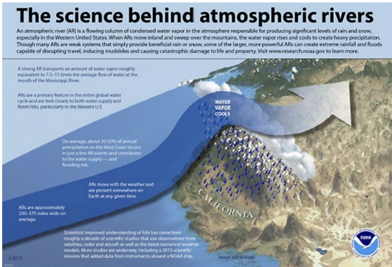
Figure 172: Diagram of an Atmospheric River Event
