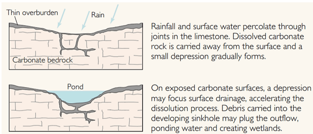
Figure 174: Dissolution Sinkhole Formation
