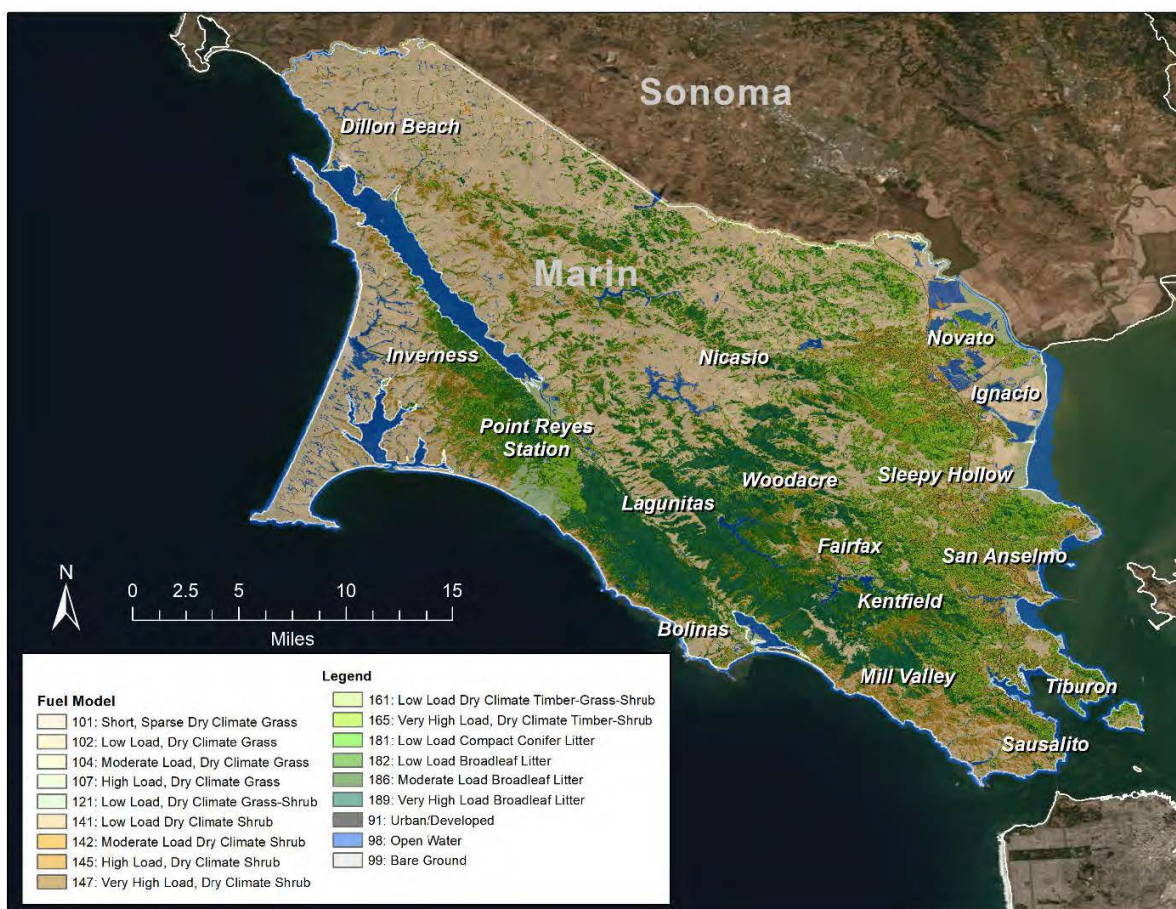
Figure 185: Fuel Model Map for the Marin County OA Source: Unknown
