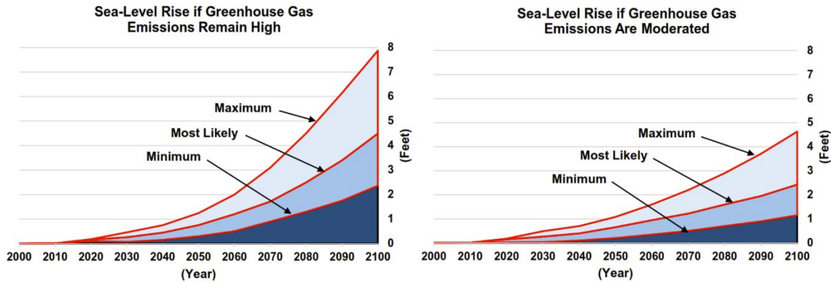
Figure 162: Projections of Sea Level Rise in the San Francisco Bay Area, 2000-2100
