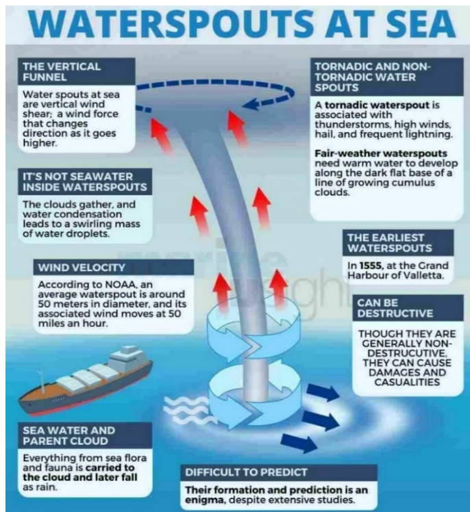
Figure 181: Waterspout Formation
