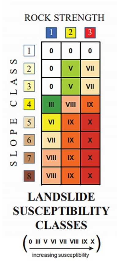
Figure 163: Landslide Susceptibility Classes Source: USGS
