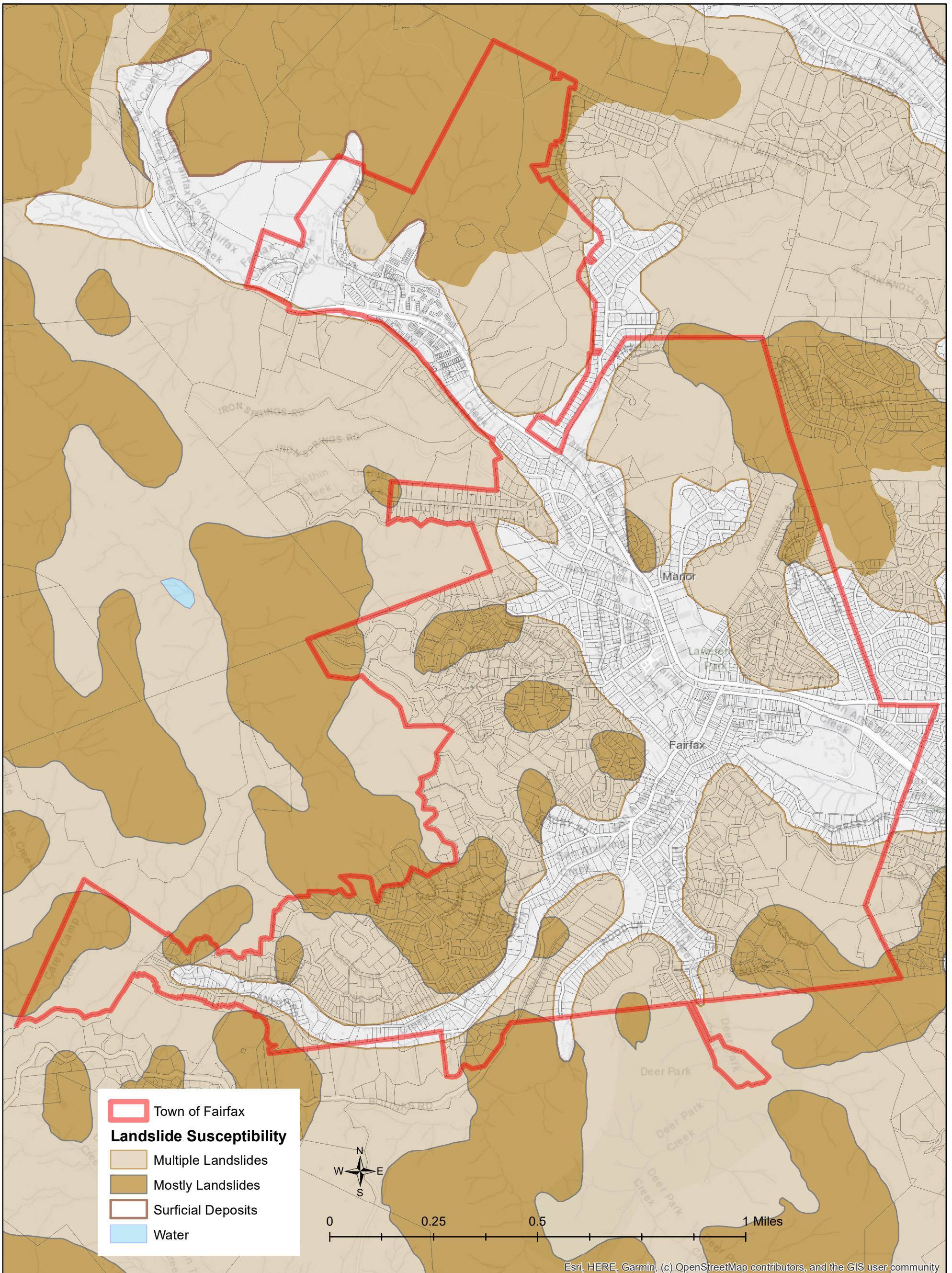
Figure S-3 Areas Susceptible to Landslides
