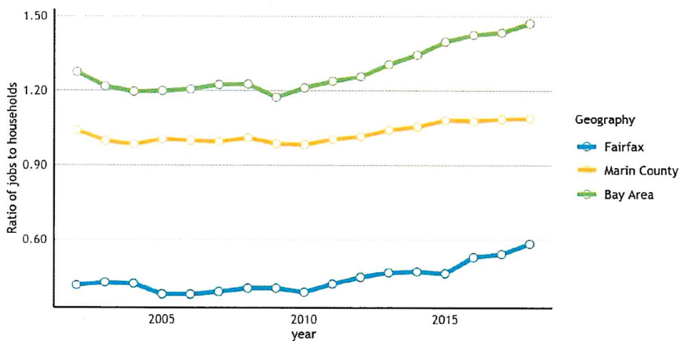
Figure 8: Jobs-Household Ratio
