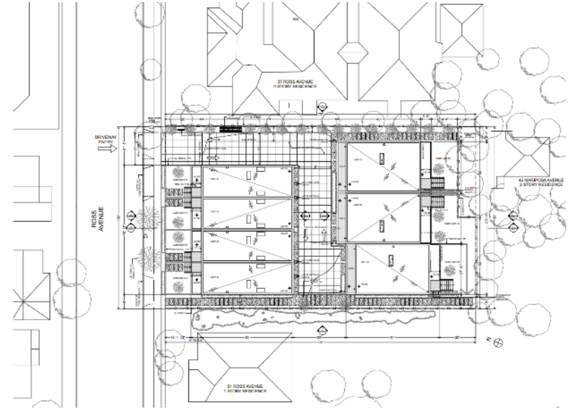
Site Plan
