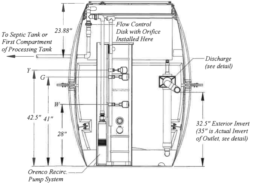
Discharge Chamber - End View
