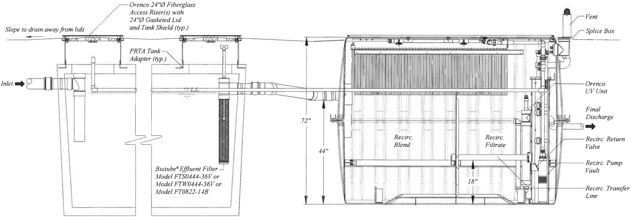
1000 gal. Primary Tank - Side View
