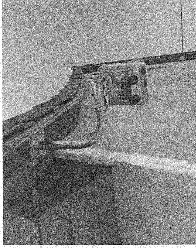
Figure 06 | Installed Terragraph receiver outside a customers home
