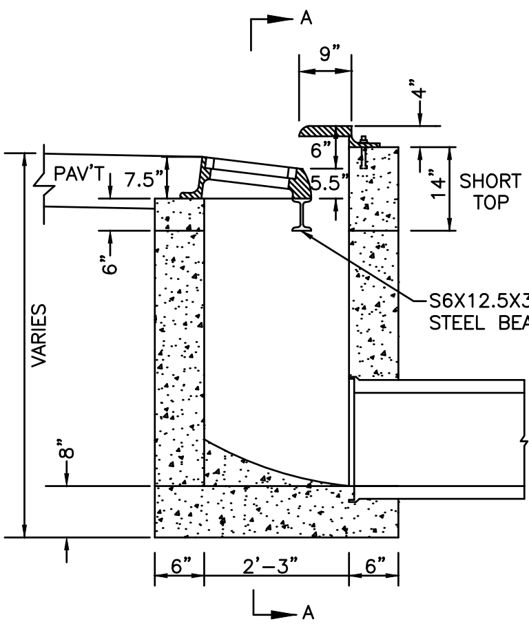
SECTION B-B
