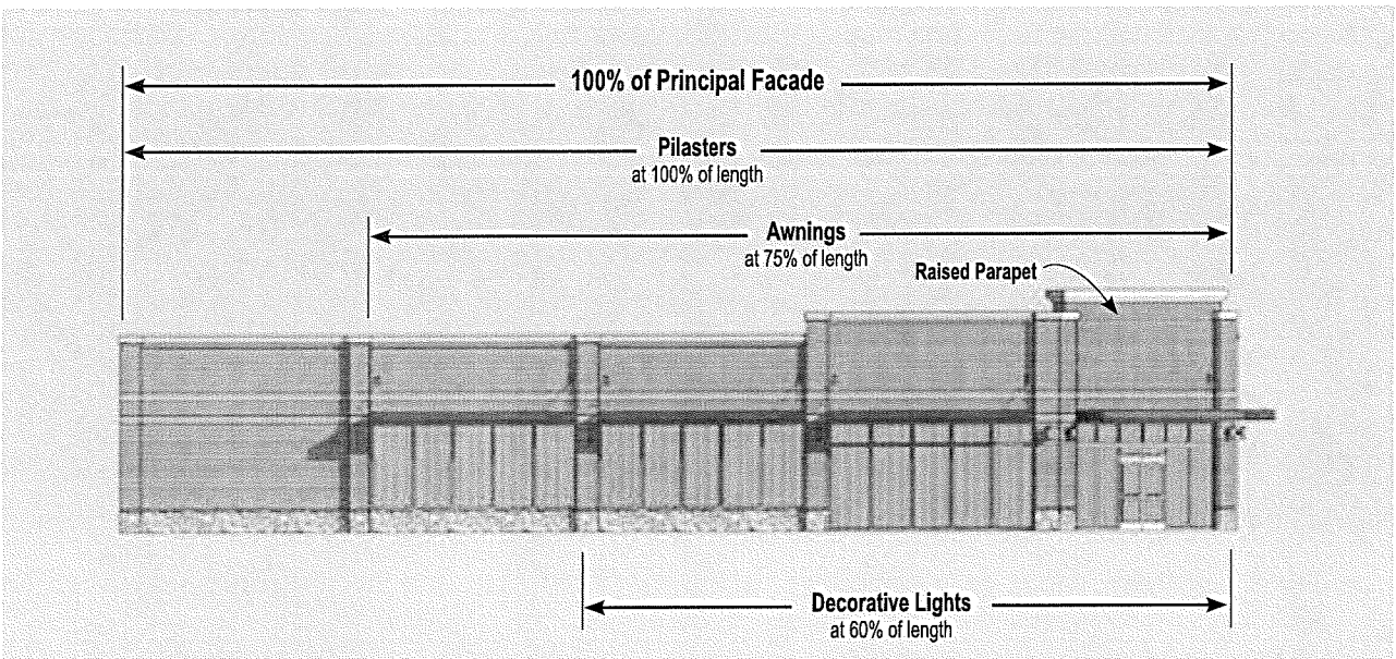
1149.03.11.I FIGURE 49.8 - MINIMUM DESIGN ELEMENTS
