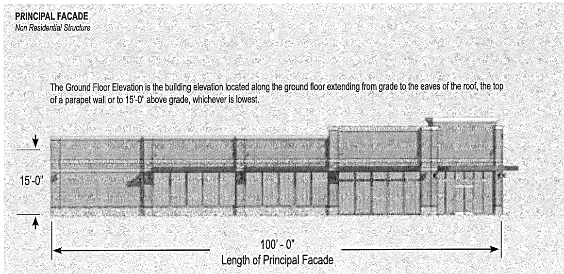
1149.03.12.D FIGURE 49.9 - MINIMUM TRANSPARENCY
