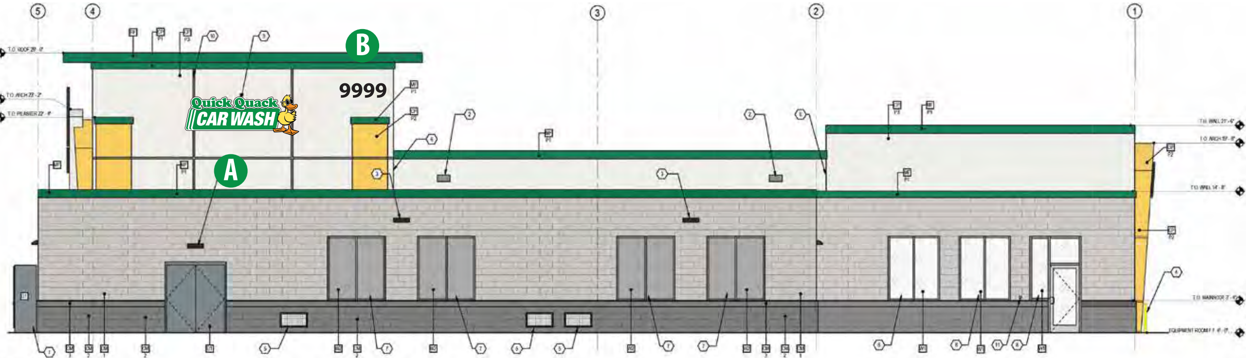
1 EAST 1/4" = 1'-0"
