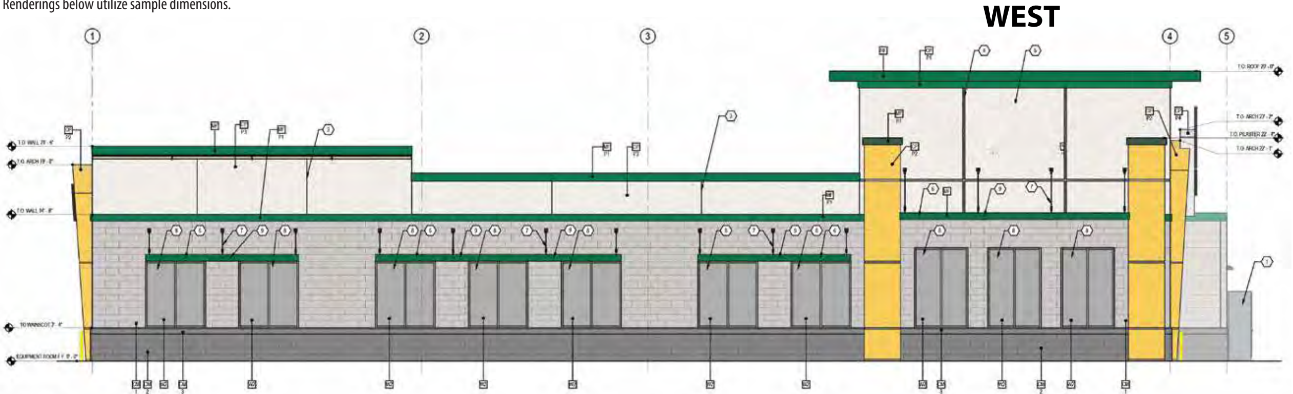
1 WEST 1/4" = 1'-0"
