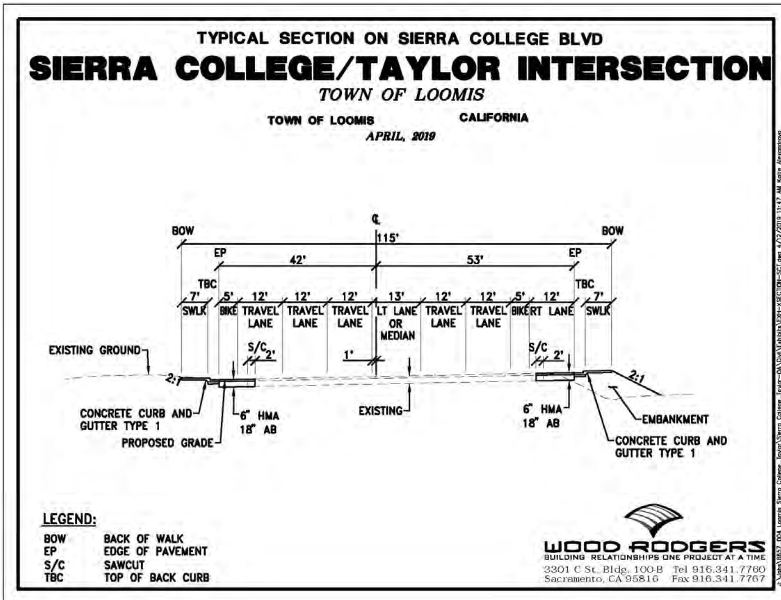
Figure 4. Roadway Cross-section
