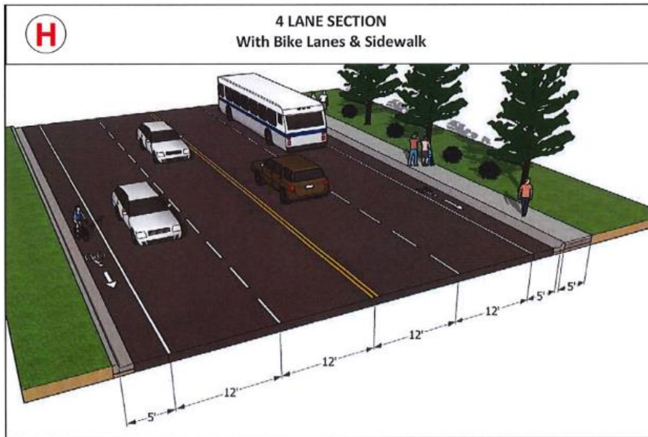
1 Figure 2-19: Roadway Cross-Sections (H)
