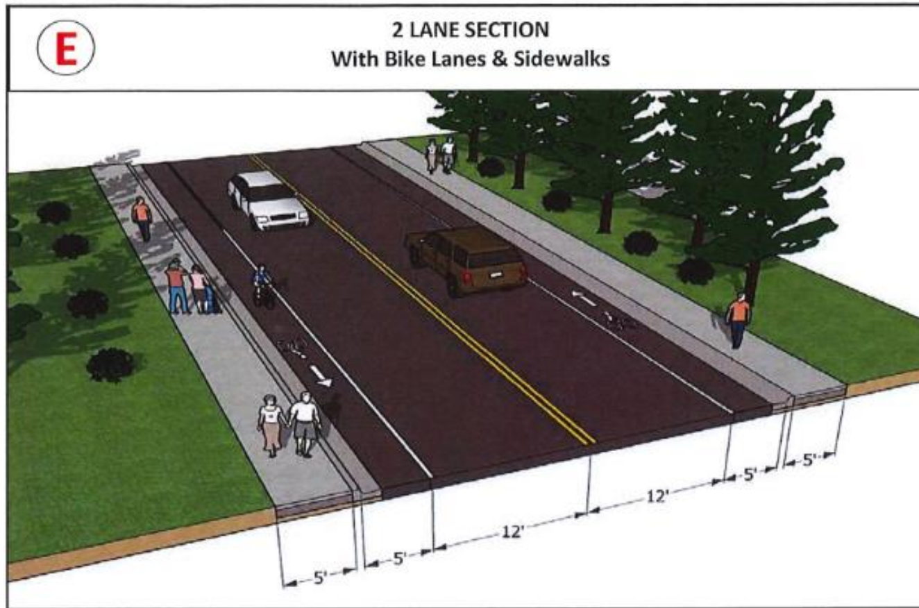
1 Figure 2-16: Roadway Cross-Sections (E)
