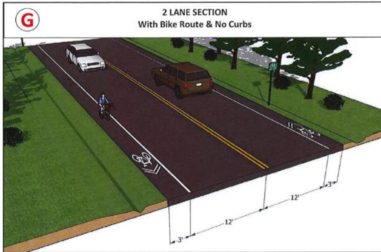
1 Figure 2-18: Roadway Cross-Sections (G)
