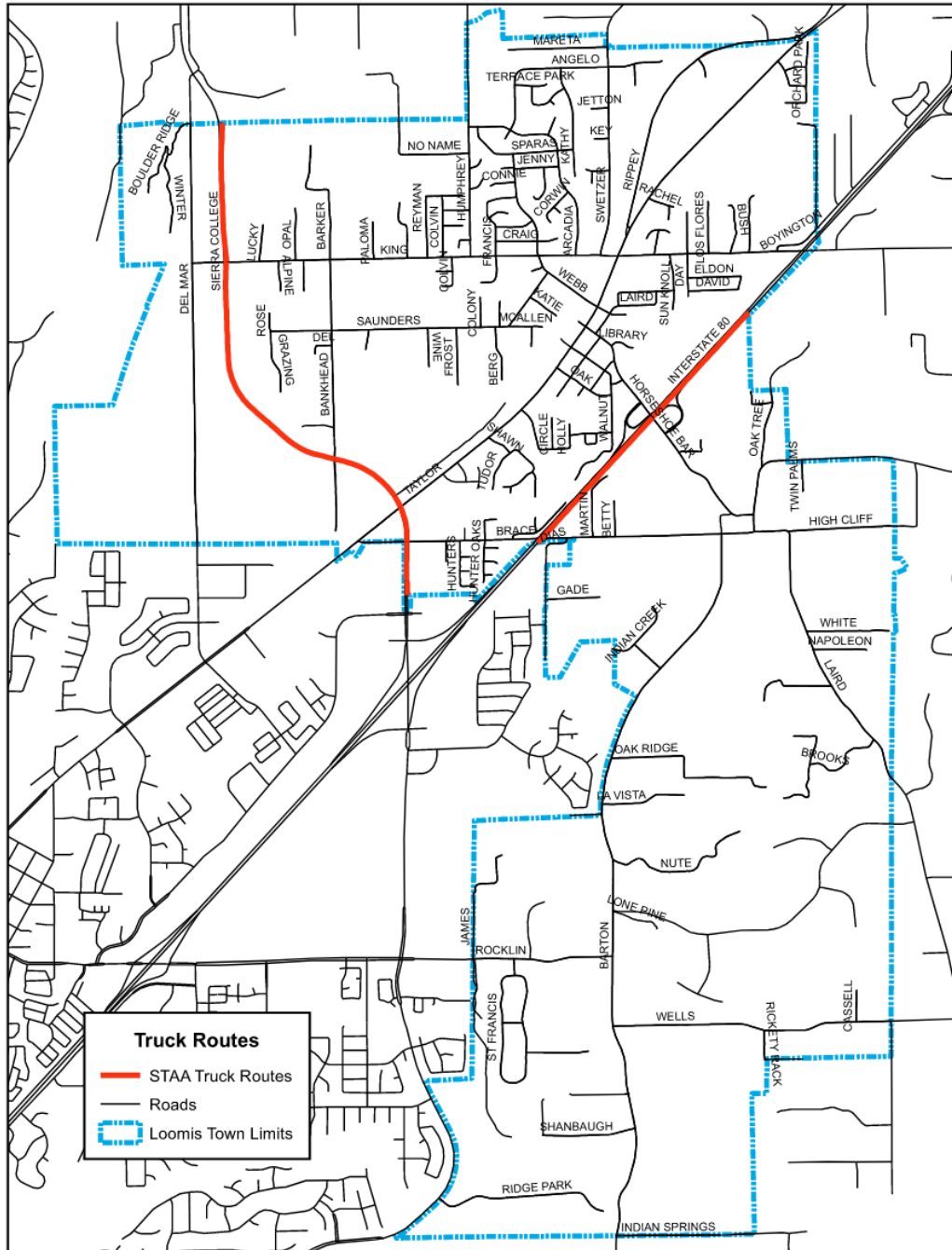
1 Figure 2-4: Existing Truck Routes
