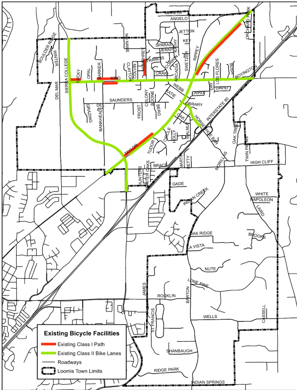
1 Figure 2-6: Existing Bicycle Facilities
