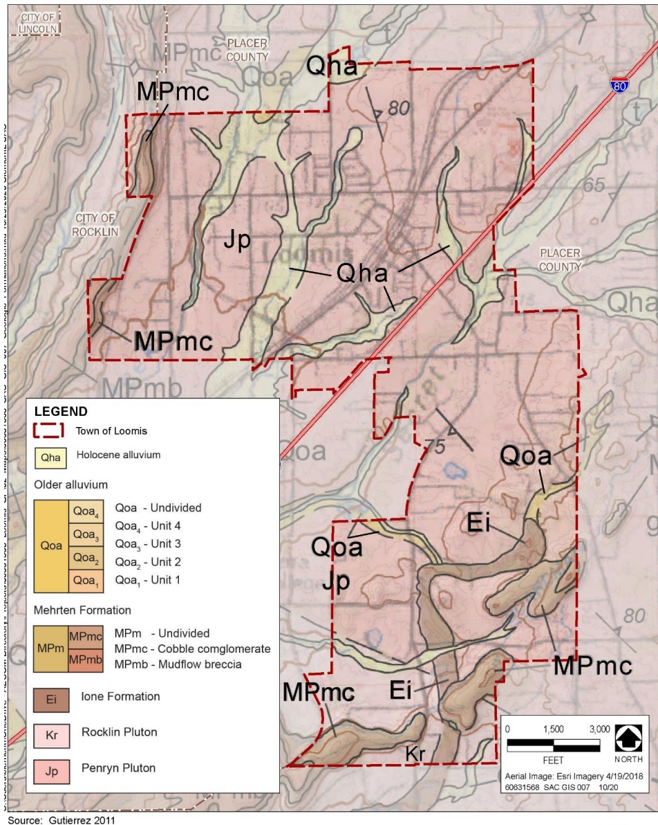
1 Figure 7-1: Geologic Map
