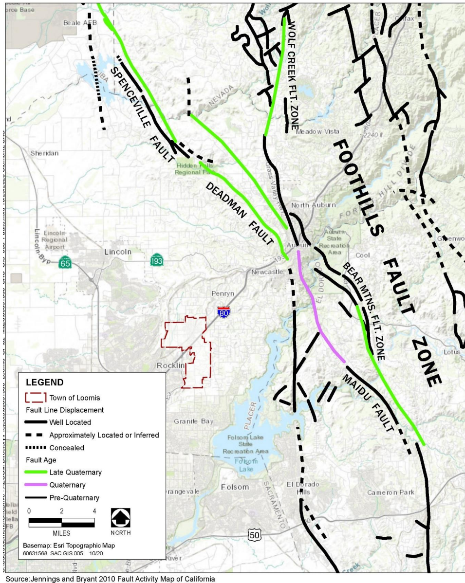
1 Figure 7-2: Regional Faults
