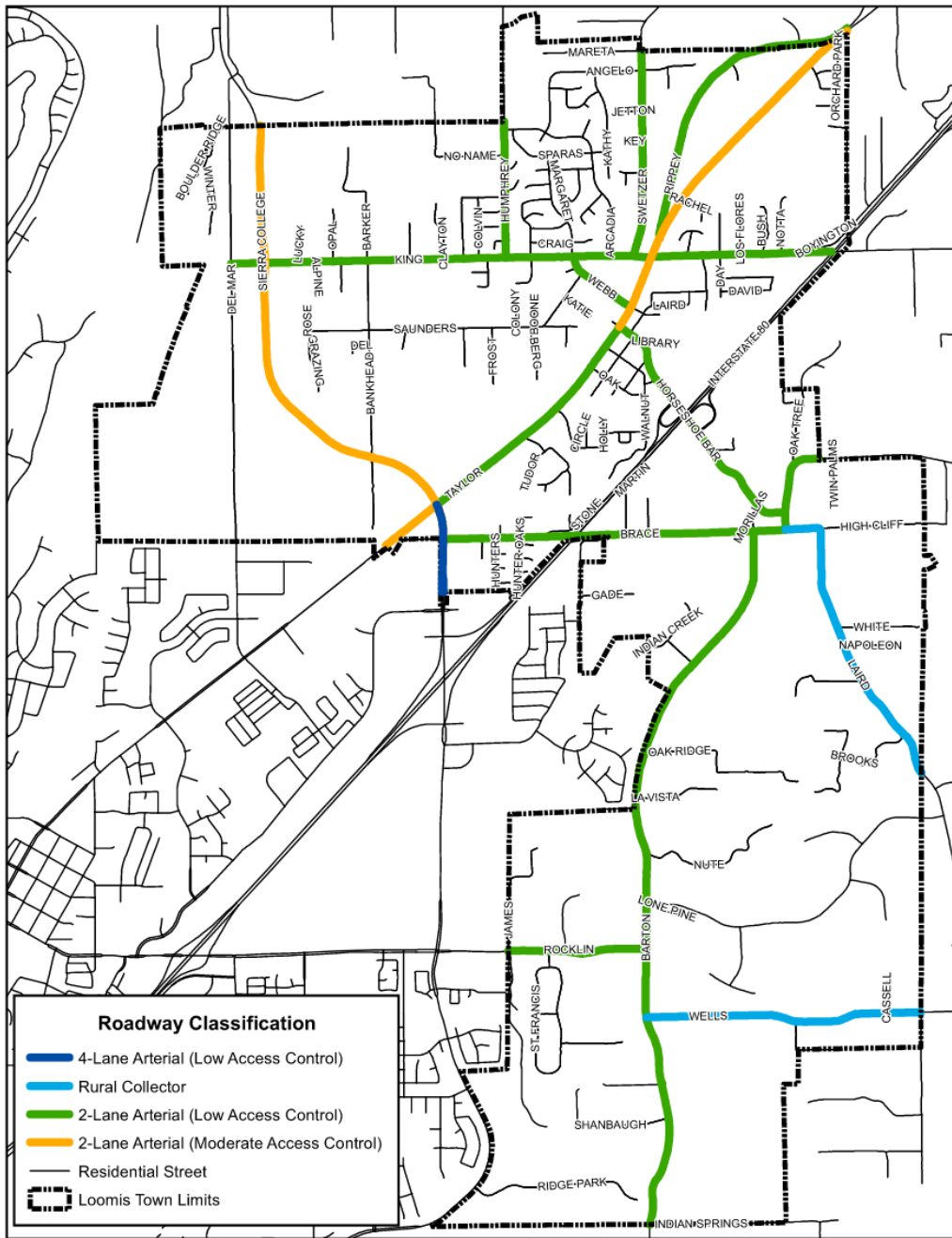
1 Figure 2-2: Existing Functional Roadway Classification Map
