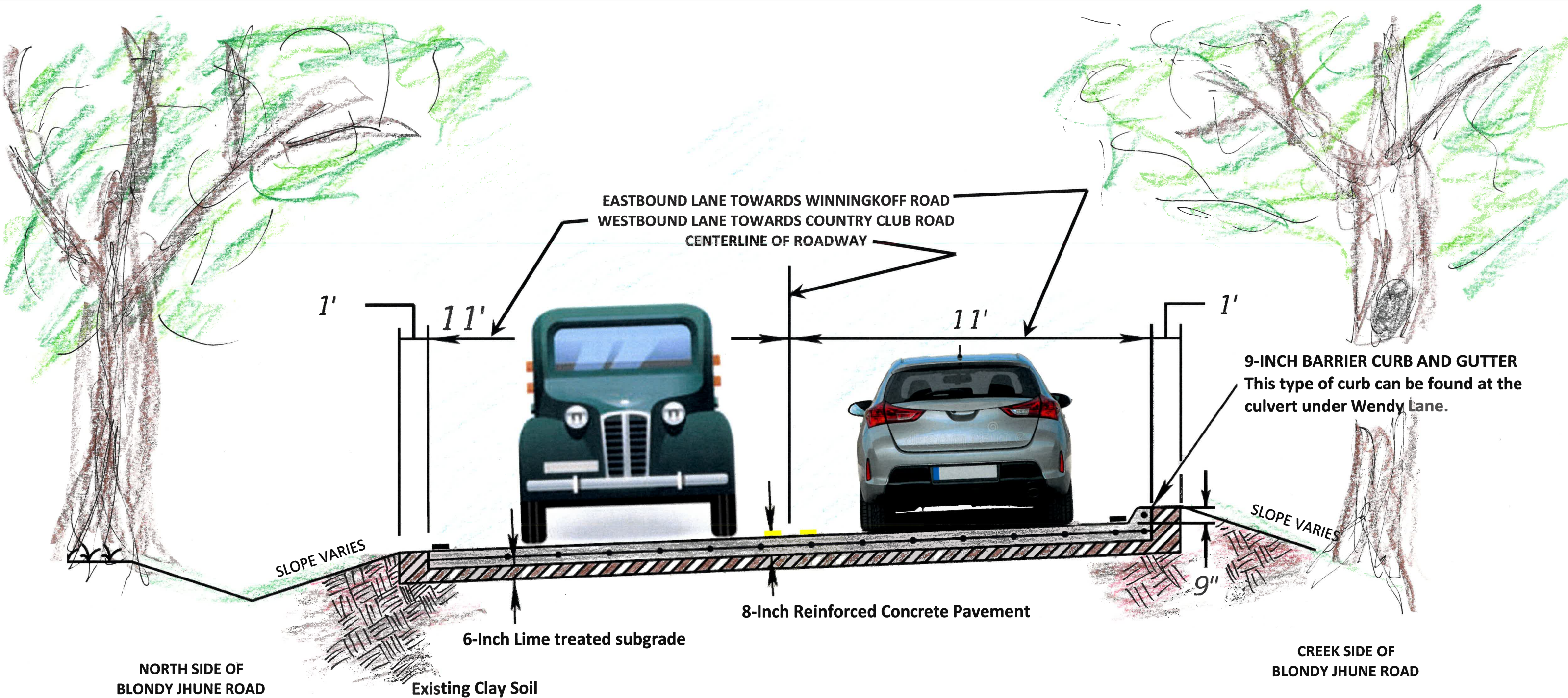
Blondy Jhune Roadway Cross Section Through the Tree Canopy
