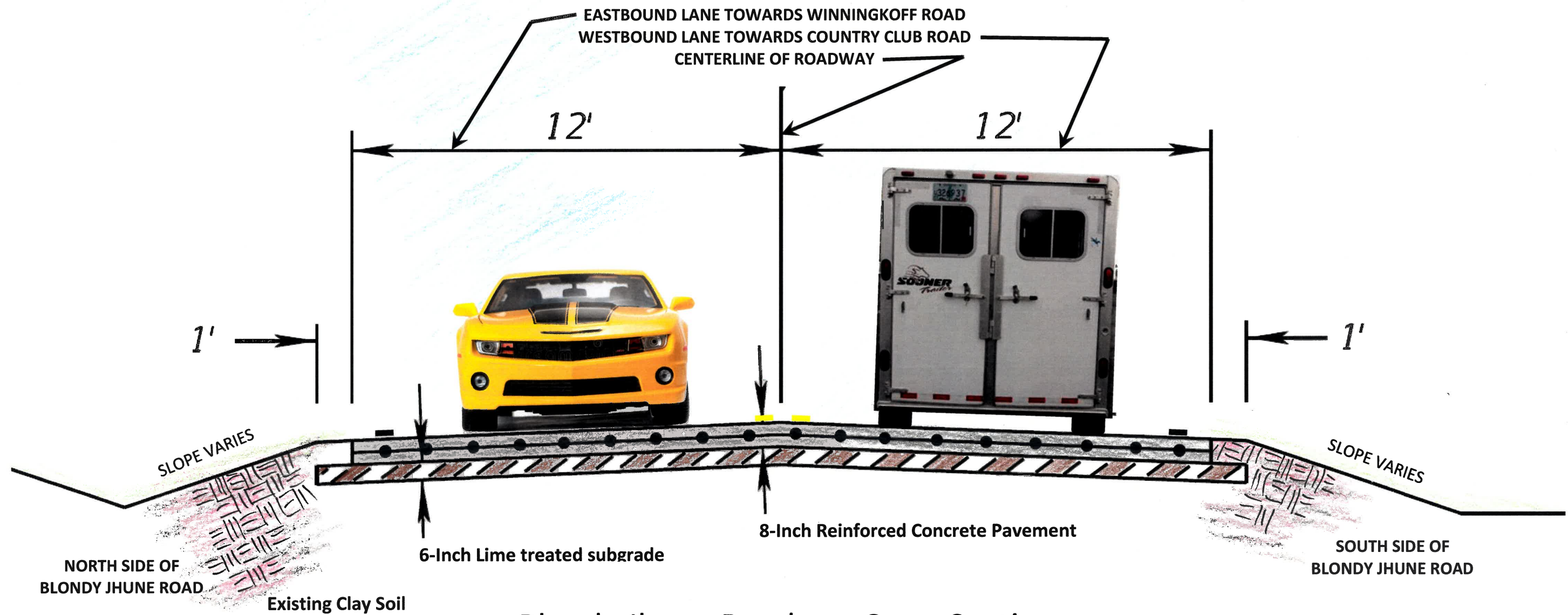
Blondy Jhune Roadway Cross Section Through the Open Areas
