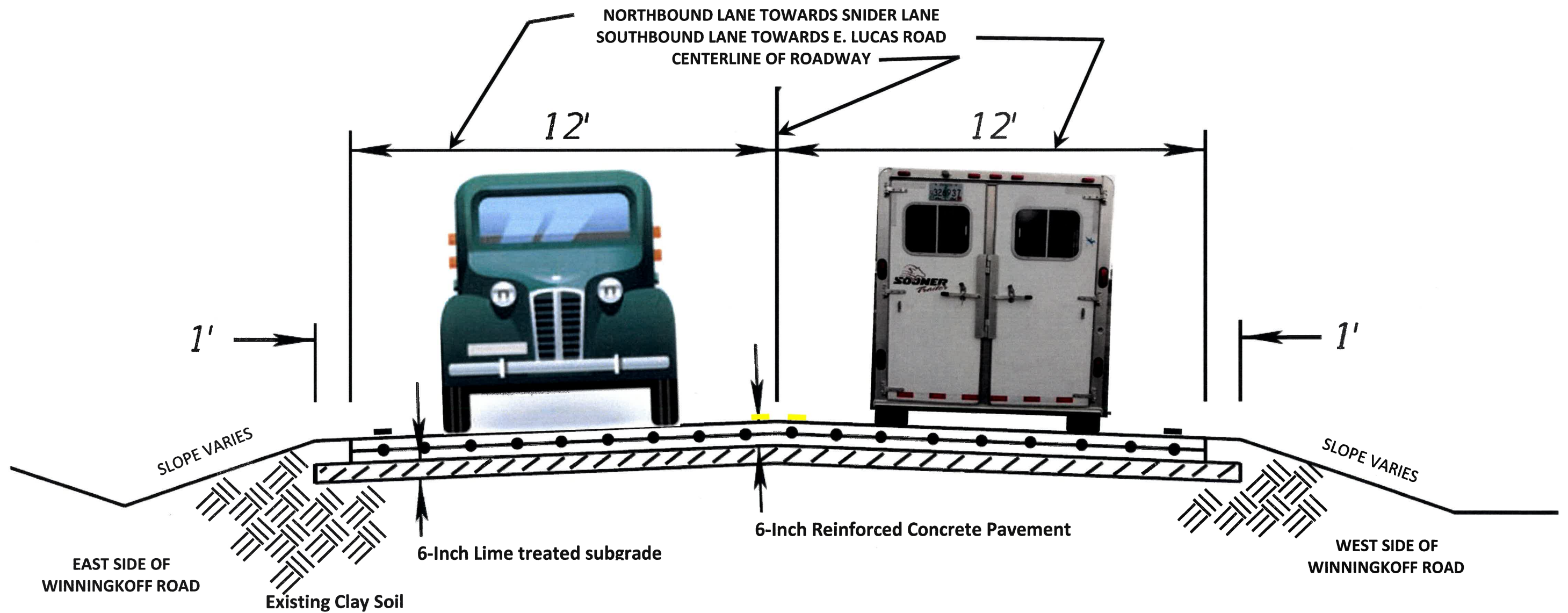
Winningkoff Roadway Cross Section
